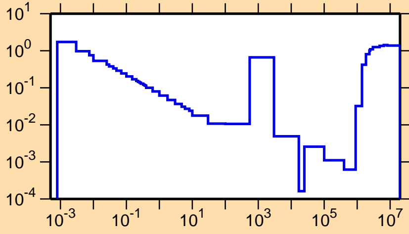
\sigma vs. E for ^{51}\text{Ti}(n,\text{nonel.})
