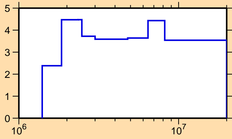
\Delta\sigma/\sigma vs. E for ^{51}\text{Ti}(n,\text{el.})
