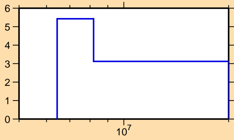
\Delta\sigma/\sigma vs. E for ^{51}\text{Ti}(n,2n)
