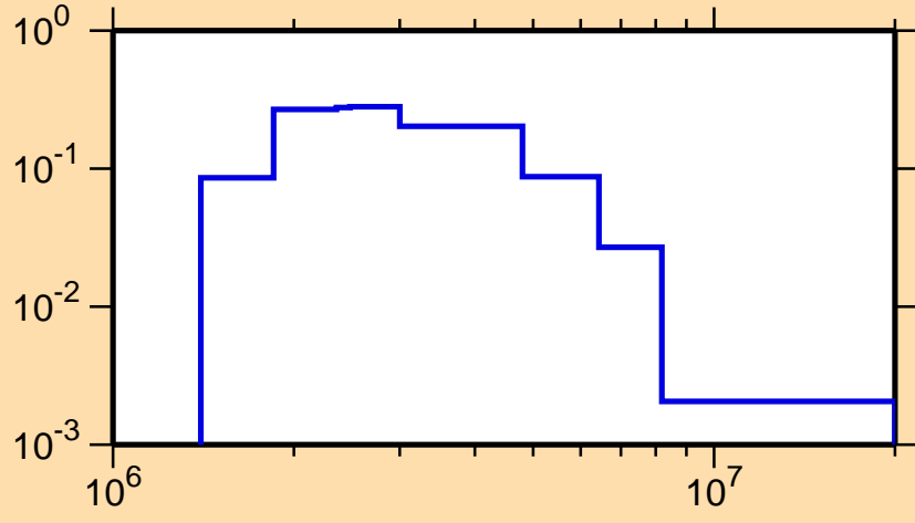
\sigma vs. E for ^{51}\text{Ti}(n,n_3)
