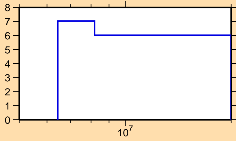
\Delta\sigma/\sigma vs. E for ^{51}\text{Ti}(n,\text{inel.})
