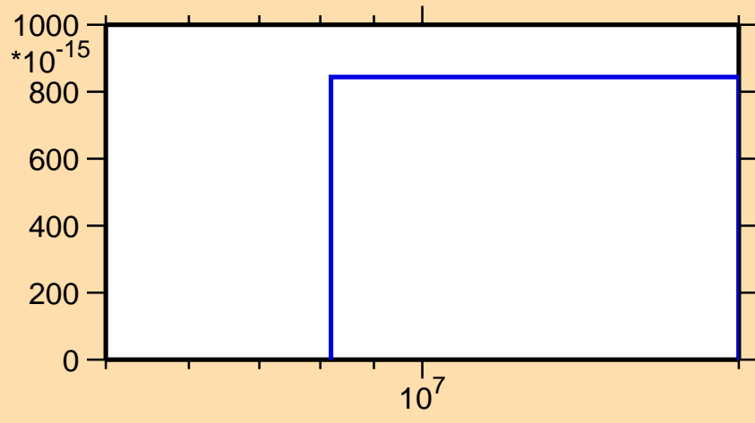
\sigma vs. E for ^{51}\text{Ti}(n,2np)
