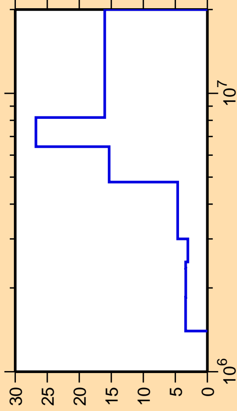
\Delta\sigma/\sigma vs. E for ^{51}\text{Ti}(n,n_3)
