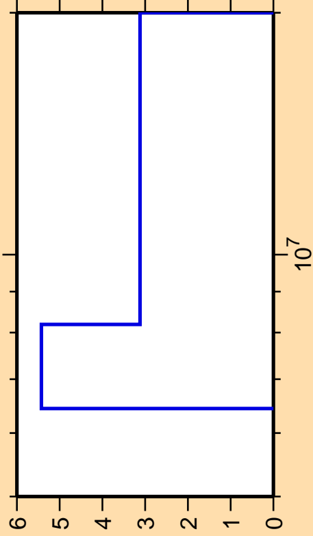
\Delta\sigma/\sigma vs. E for ^{51}\text{Ti}(n,2n)
