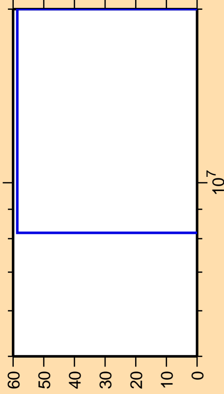
\Delta\sigma/\sigma vs. E for ^{51}\text{Ti}(n,nd)
