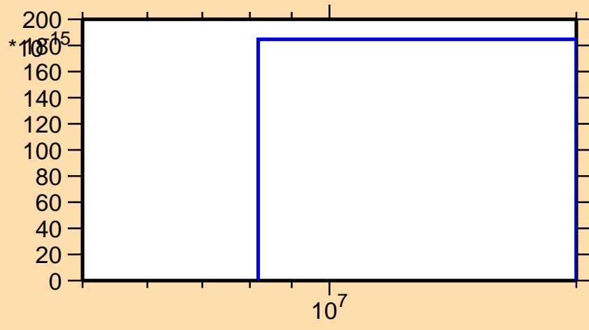
\sigma vs. E for ^{51}\text{Ti}(n,\text{He}3)
