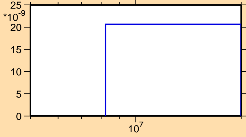
\sigma vs. E for ^{51}\text{Ti}(n,nd)
