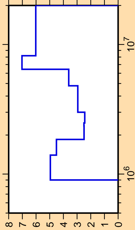
\Delta\sigma/\sigma vs. E for ^{51}\text{Ti}(n,\text{inel.})
