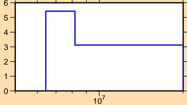
\Delta\sigma/\sigma vs. E for ^{51}\text{Ti}(n,2n)
