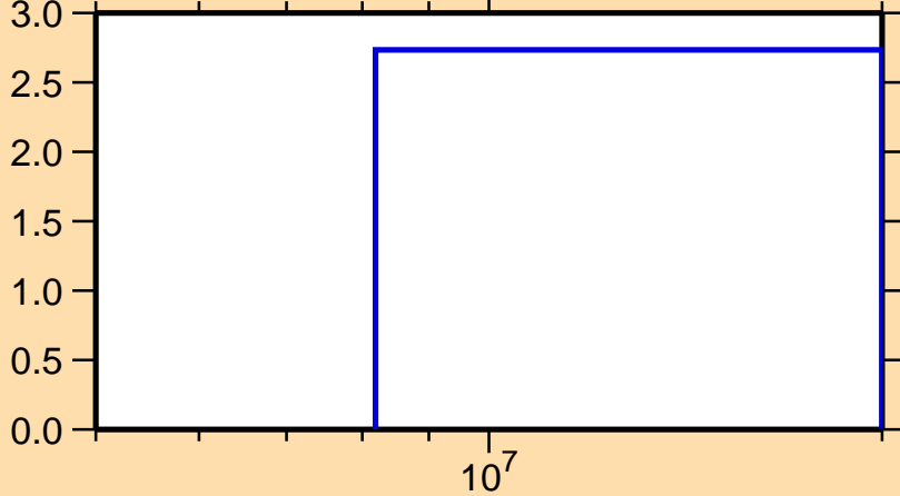
\Delta\sigma/\sigma vs. E for ^{52}\text{Ti}(n,\text{nonel.})
