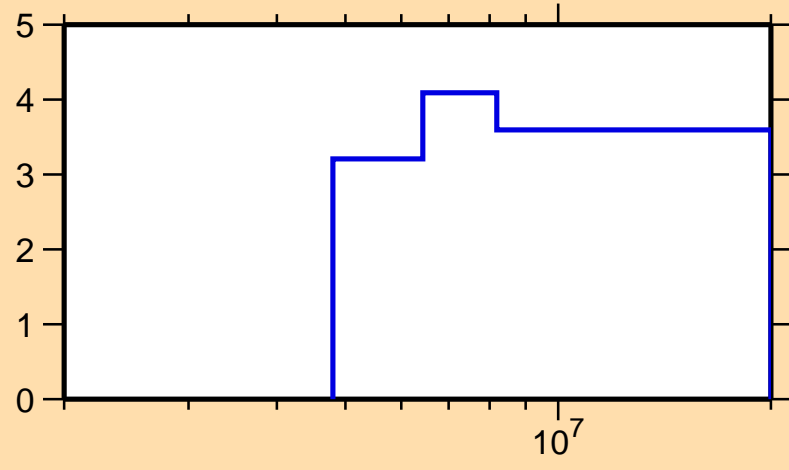
\Delta\sigma/\sigma vs. E for ^{52}\text{Ti}(n,\text{tot.})
