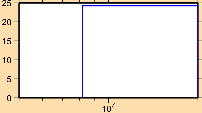
\Delta\sigma/\sigma vs. E for ^{52}\text{Ti}(n,\gamma)
