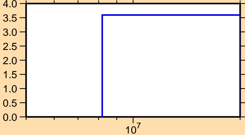
\Delta\sigma/\sigma vs. E for ^{52}\text{Ti}(n,\text{tot.})
