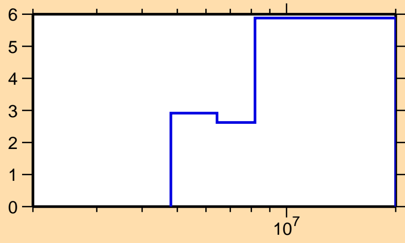
\Delta\sigma/\sigma vs. E for ^{52}\text{Ti}(n,\text{inel.})
