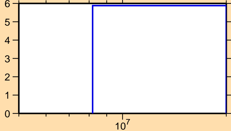
\Delta\sigma/\sigma vs. E for ^{52}\text{Ti}(n,\text{inel.})
