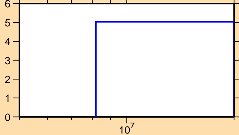
\Delta\sigma/\sigma vs. E for ^{52}\text{Ti}(n,el.)
