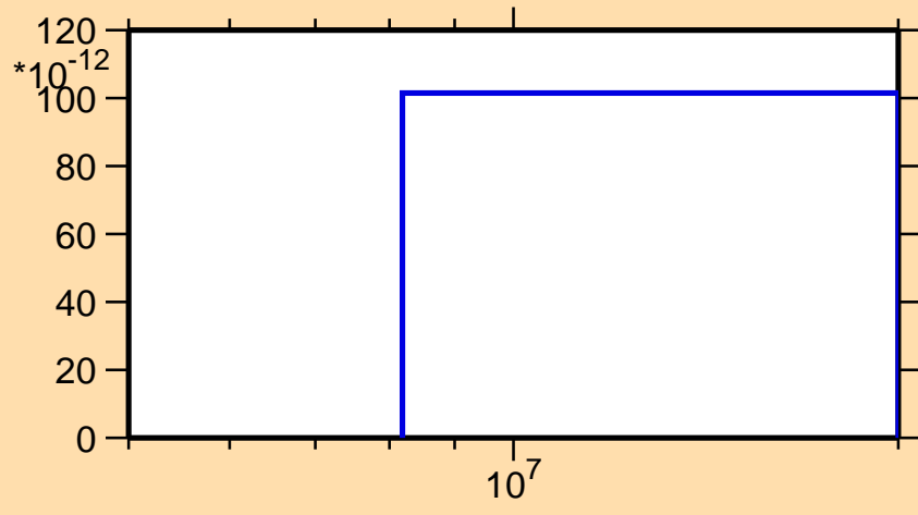
\sigma vs. E for ^{53}\text{Ti}(n,nt)
