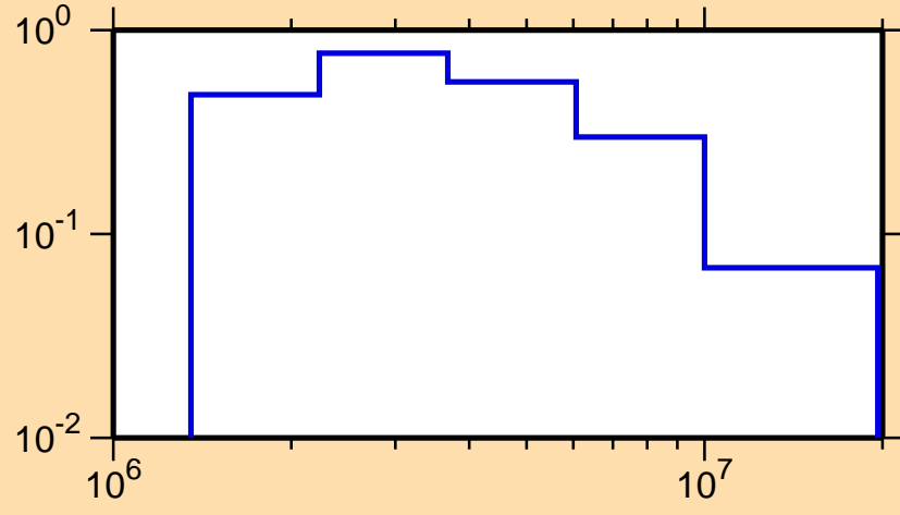
\sigma vs. E for ^{54}\text{Ti}(n,n_1)
