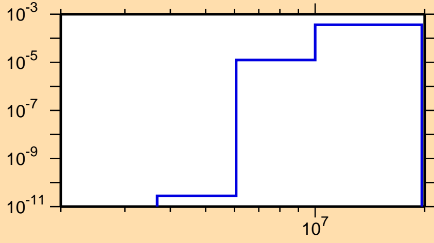
\sigma vs. E for ^{54}\text{Ti}(n,\alpha)
