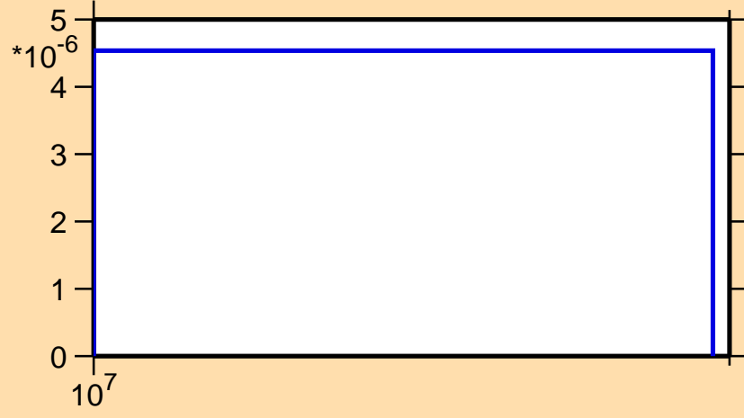
\sigma vs. E for ^{54}\text{Ti}(n,np)
