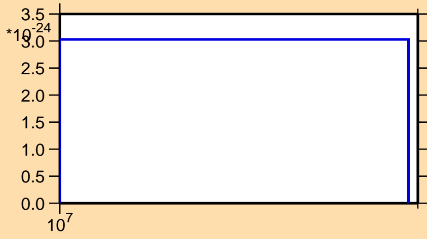
\sigma vs. E for ^{54}\text{Ti}(n,\text{He}3)
