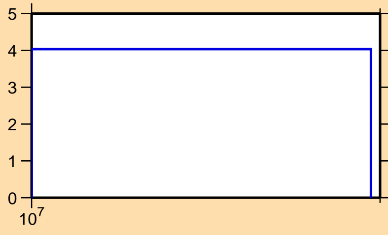
\Delta\sigma/\sigma vs. E for ^{54}\text{Ti}(n,\text{tot.})
