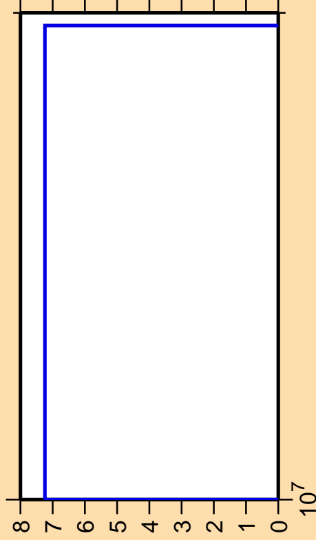
\Delta\sigma/\sigma vs. E for ^{54}\text{Ti}(n,\text{nd})
