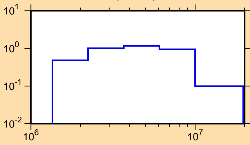
\sigma vs. E for ^{54}\text{Ti}(n,\text{inel.})
