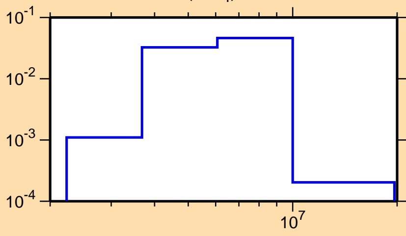
\sigma vs. E for ^{54}\text{Ti}(n,n_4)
