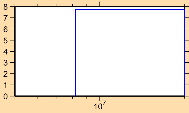
\Delta\sigma/\sigma vs. E for ^{54}\text{Ti}(n,el.)
