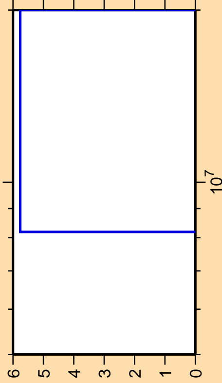
\Delta\sigma/\sigma vs. E for ^{54}\text{Ti}(n,nd)
