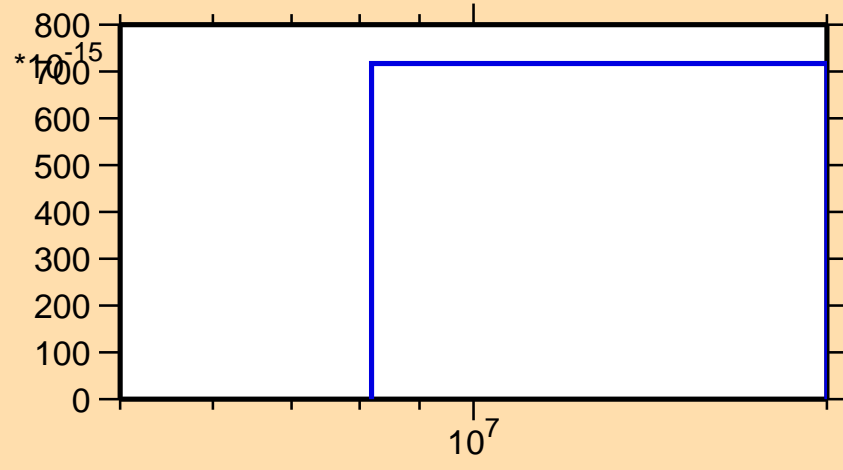
\sigma vs. E for ^{54}\text{Ti}(n,nd)
