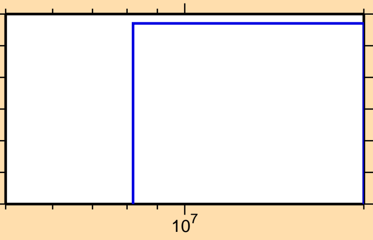
\sigma vs. E for ^{54}\text{Ti}(n,p)
