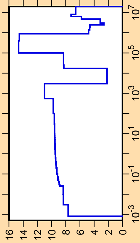
\Delta\sigma/\sigma vs. E for ^{55}\text{Ti}(n,\text{tot.})
