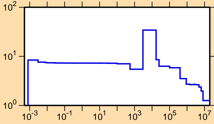
\sigma vs. E for ^{55}\text{Ti}(n,\text{el.})
