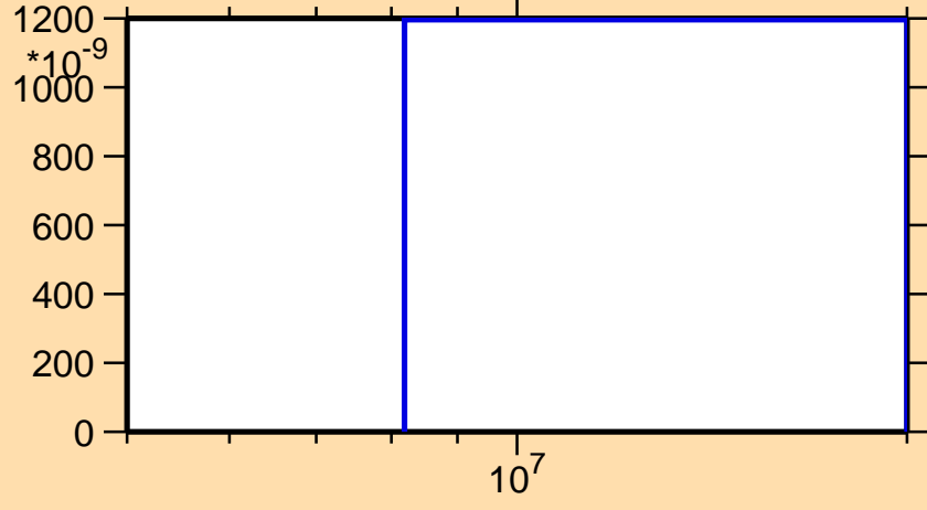
\sigma vs. E for ^{55}\text{Ti}(n,np)
