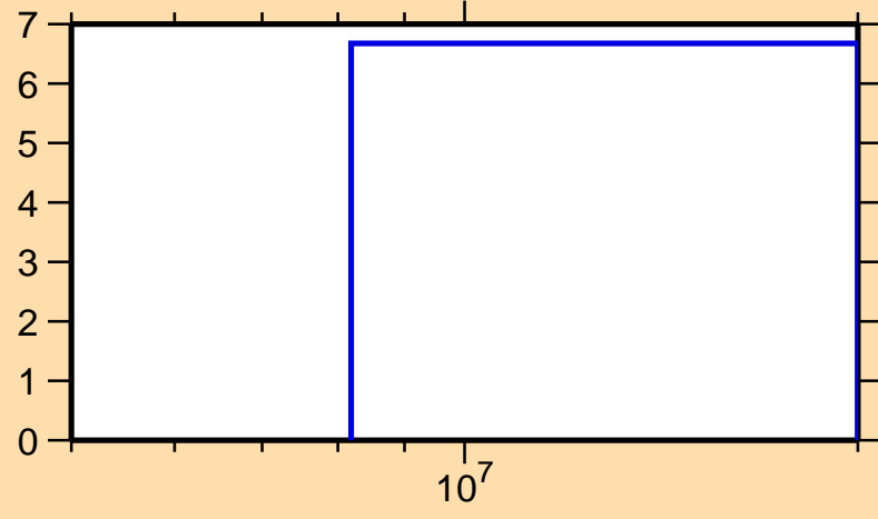
\Delta\sigma/\sigma vs. E for ^{55}\text{Ti}(n,2n)
