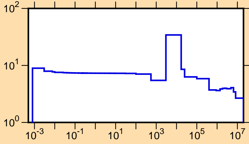
\sigma vs. E for ^{55}\text{Ti}(n,\text{tot.})
