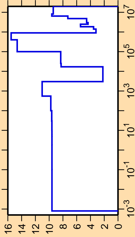
\Delta\sigma/\sigma vs. E for ^{55}\text{Ti}(n,\text{el.})
