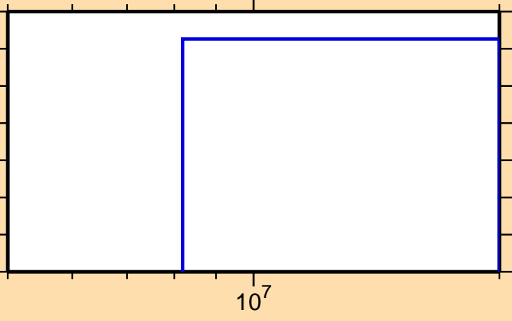
\sigma vs. E for ^{55}\text{Ti}(n,3n)
