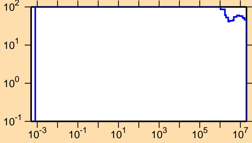
\Delta\sigma/\sigma vs. E for ^{180}\text{Tl}(n,p)
