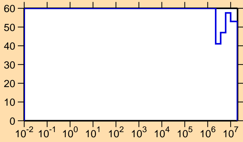
\Delta\sigma/\sigma vs. E for ^{180}\text{Tl}(n,p)
