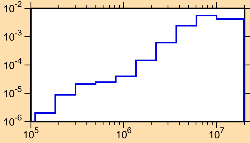
\sigma vs. E for ^{180}\text{Tl}(n,n\alpha)
