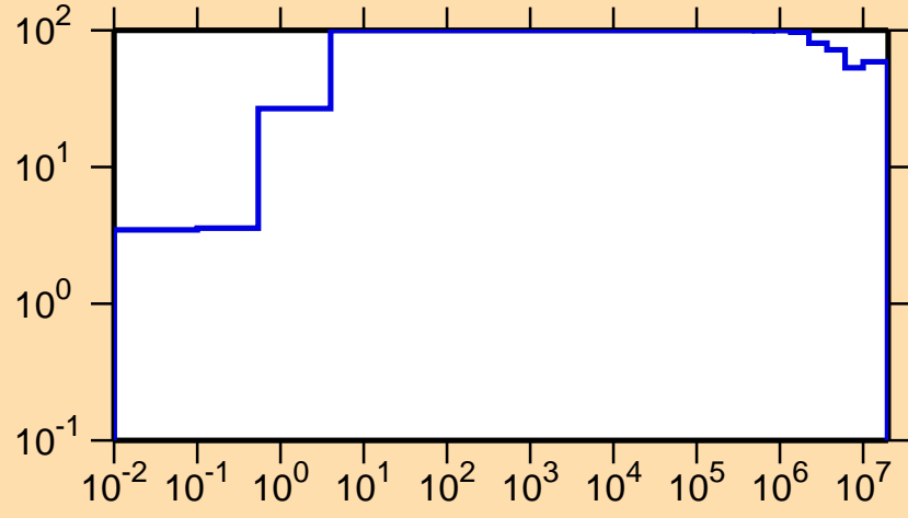
\Delta\sigma/\sigma vs. E for ^{180}\text{Tl}(n,\gamma)
