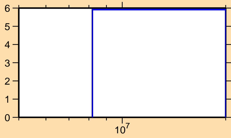
\Delta\sigma/\sigma vs. E for ^{180}\text{Tl}(n,\text{tot.})
