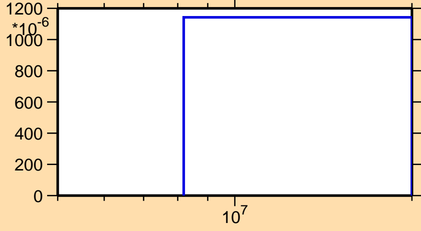
\sigma vs. E for ^{180}\text{Tl}(n,2n)
