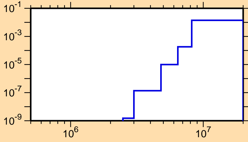
\sigma vs. E for ^{180}\text{Tl}(n,d)
