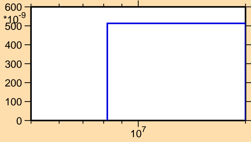
\sigma vs. E for ^{180}\text{Tl}(n,nd)
