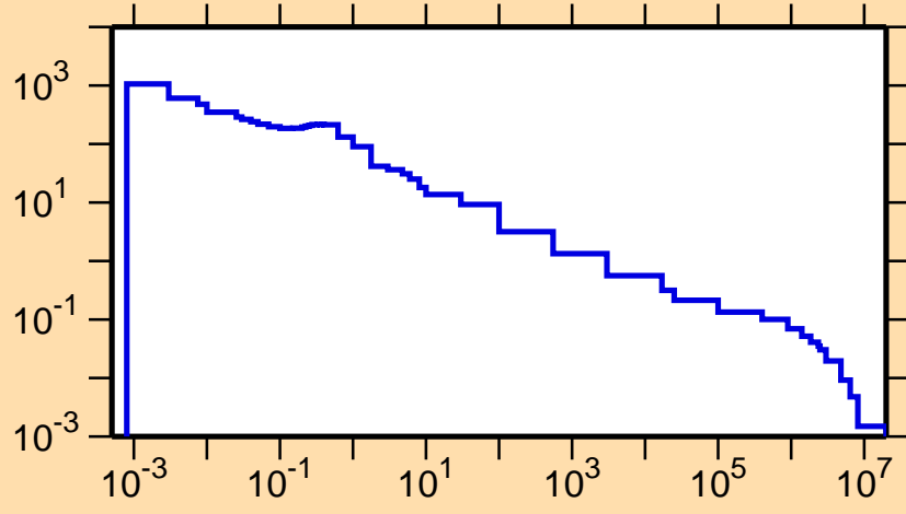
\sigma vs. E for ^{180}\text{Tl}(n,\gamma)
