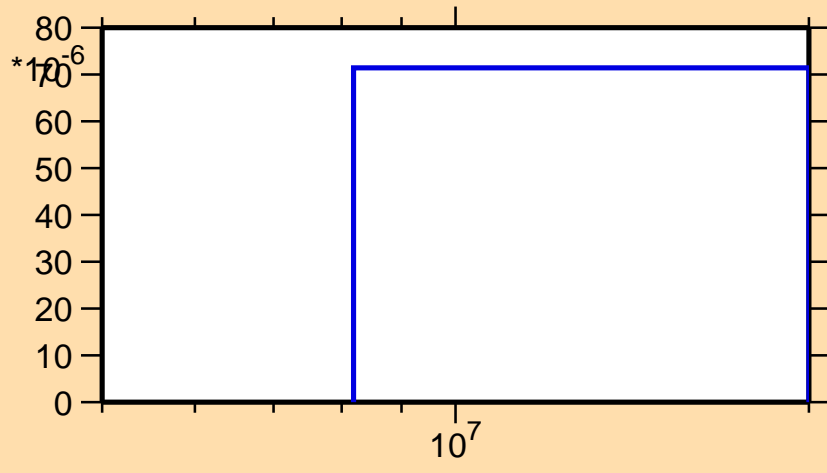
\sigma vs. E for ^{180}\text{Tl}(n,2np)
