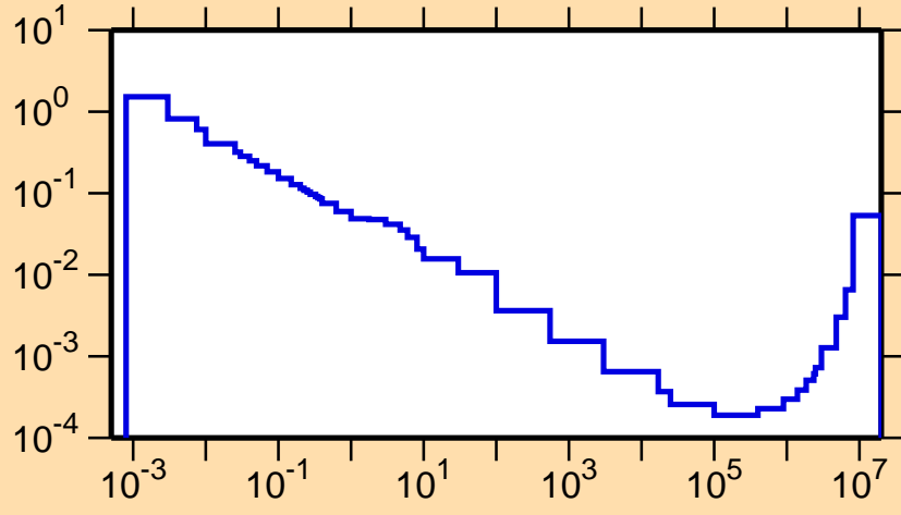
\sigma vs. E for ^{180}\text{Tl}(n,p\alpha)
