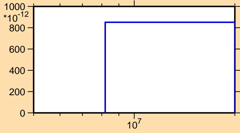
\sigma vs. E for ^{180}\text{Tl} (mt 34)
