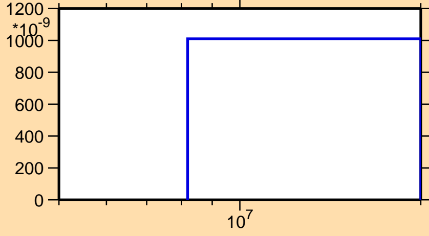
\sigma vs. E for ^{180}\text{Tl}(n,\text{pt})
