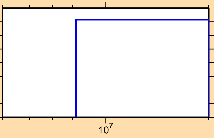
\sigma vs. E for ^{180}\text{Tl}(n,2np)
