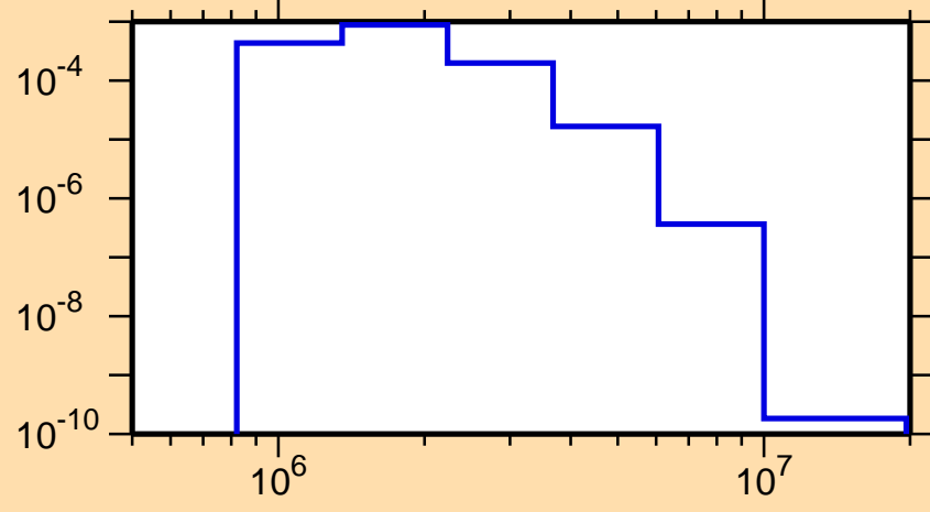
\sigma vs. E for ^{181}\text{Tl}(n,n_3)
