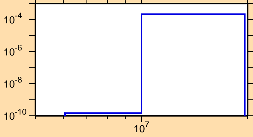
\sigma vs. E for ^{181}\text{Tl}(n,t)
