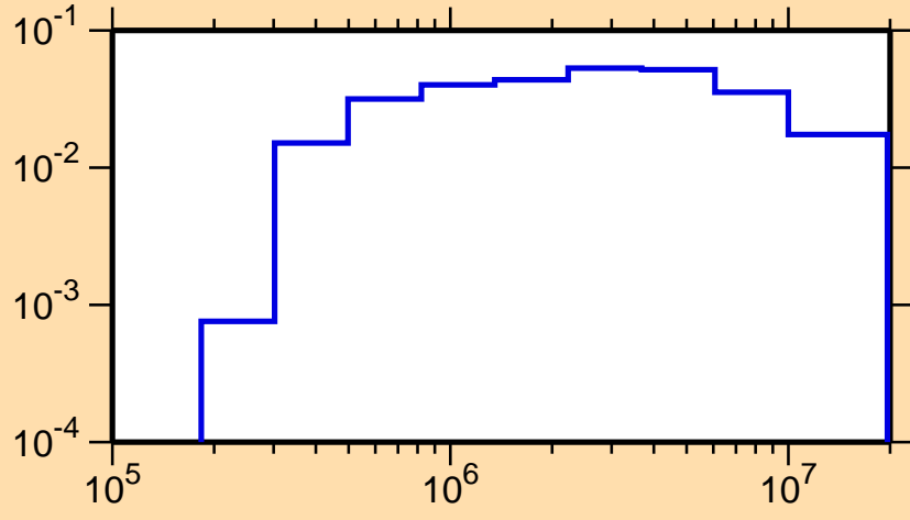
\sigma vs. E for ^{181}\text{Tl}(n,n_1)
