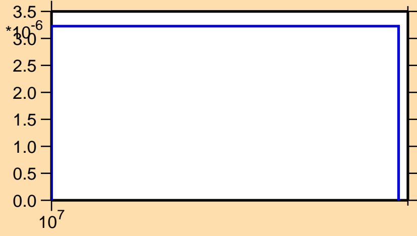
\sigma vs. E for ^{181}\text{Tl}(n,2np)
