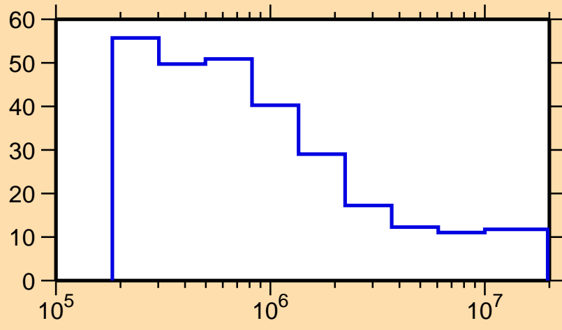
\Delta\sigma/\sigma vs. E for ^{181}\text{Tl}(n,\text{nonel.})
