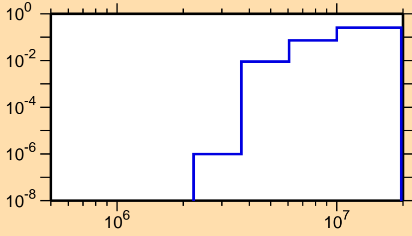
\sigma vs. E for ^{181}\text{Tl}(n,np)
