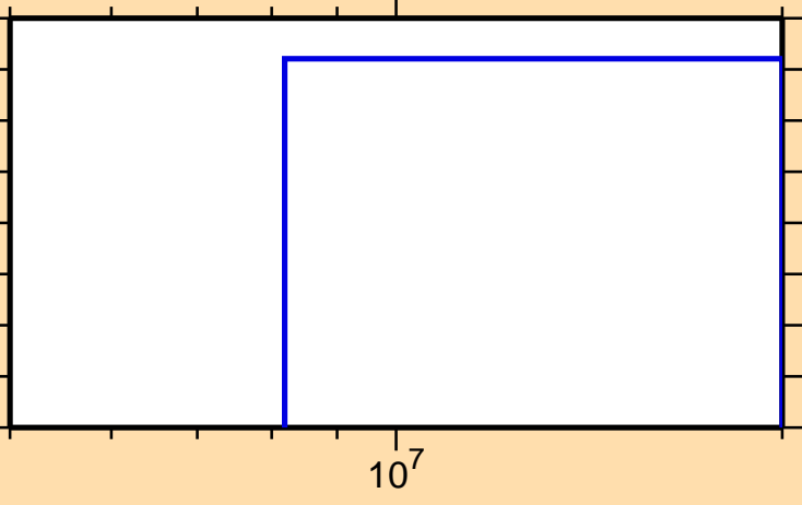
\sigma vs. E for ^{181}\text{Tl} (mt 34)
