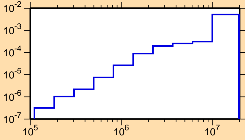
\sigma vs. E for ^{182}\text{Tl}(n,n\alpha)
