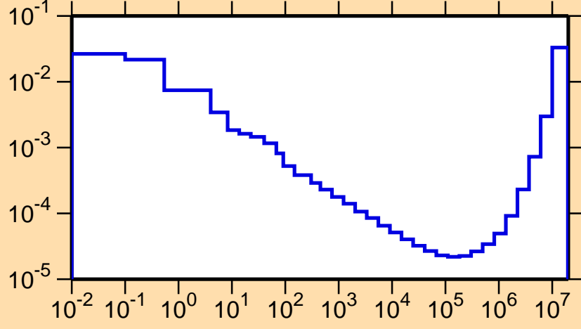
\sigma vs. E for ^{182}\text{Tl}(n,p\alpha)
