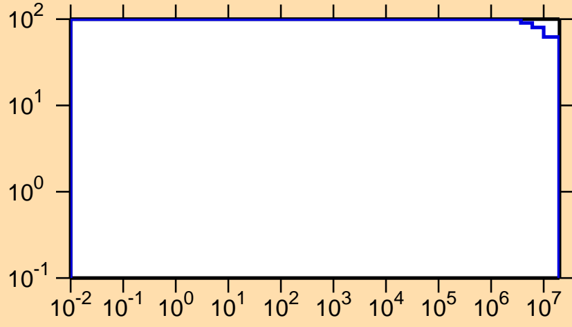
\Delta\sigma/\sigma vs. E for ^{182}\text{Tl}(n,p)
