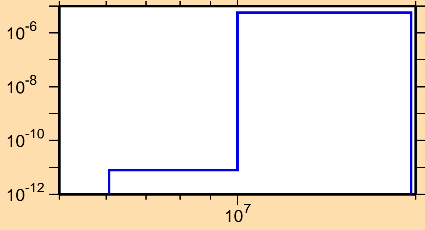
\sigma vs. E for ^{182}\text{Tl}(n,pd)
