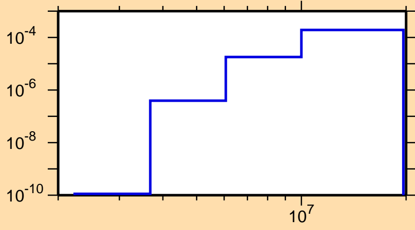
\sigma vs. E for ^{182}\text{Tl} (mt 45)
