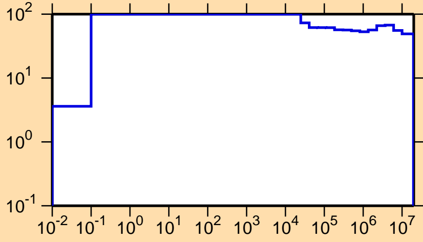
\Delta\sigma/\sigma vs. E for ^{182}\text{Tl}(n,\gamma)
