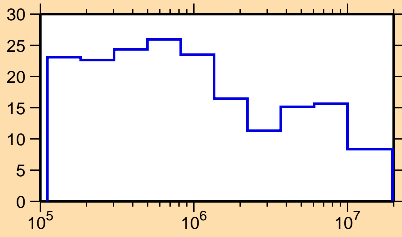
\Delta\sigma/\sigma vs. E for ^{182}\text{Tl}(n,\text{tot.})
