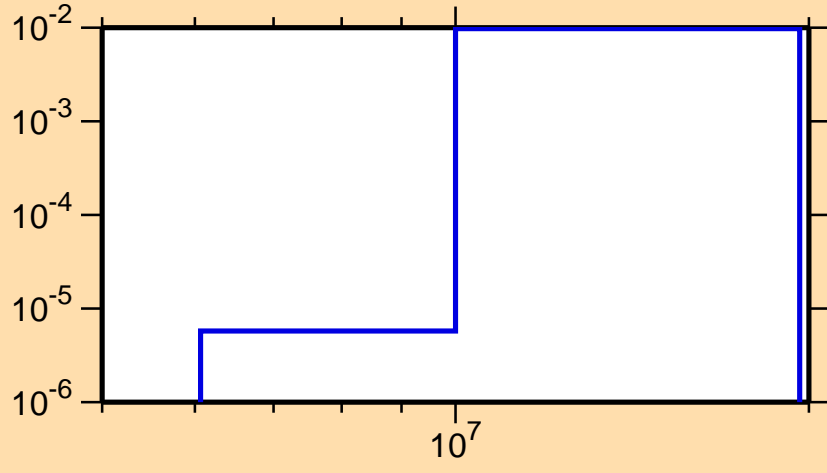
\sigma vs. E for ^{182}\text{Tl}(n,2n)
