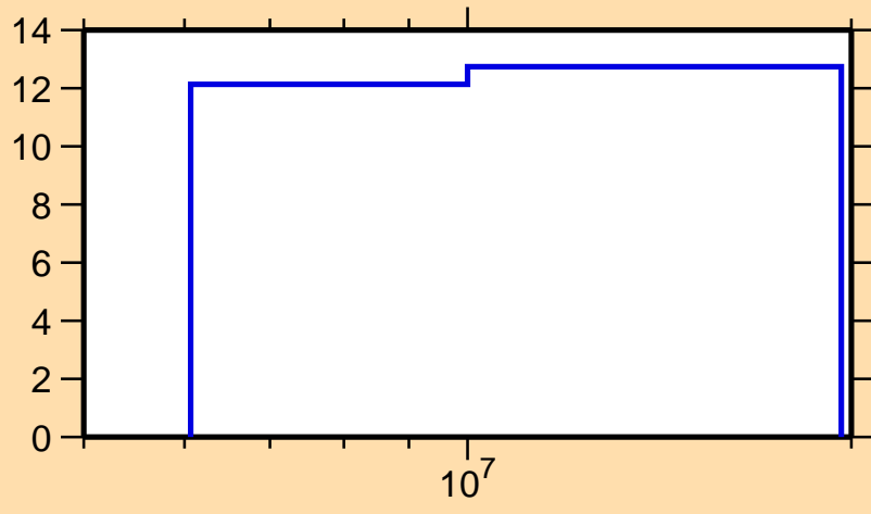
\Delta\sigma/\sigma vs. E for ^{182}\text{Tl}(n,\text{nonel.})
