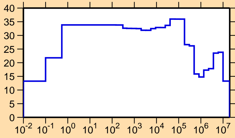
\Delta\sigma/\sigma vs. E for ^{182}\text{Tl}(n,\text{el.})
