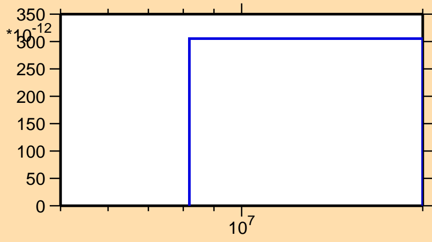
\sigma vs. E for ^{182}\text{Tl} (mt 34)
