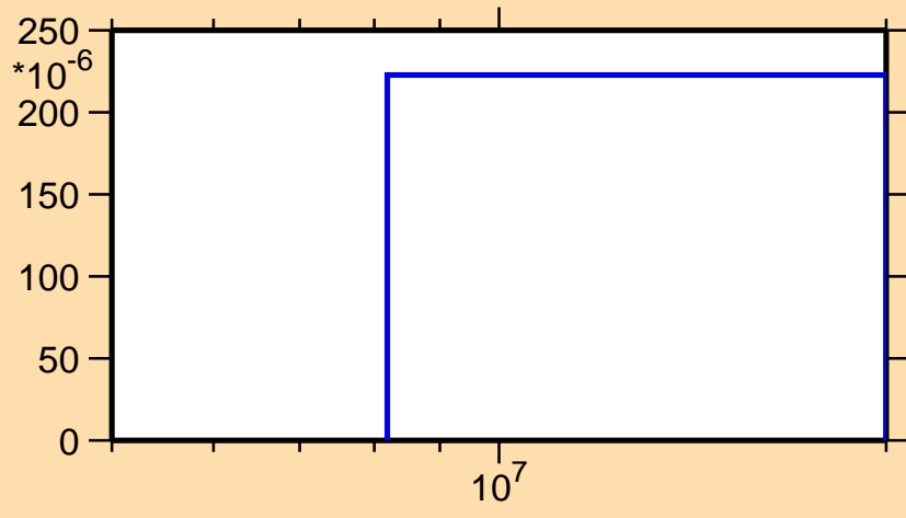
\sigma vs. E for ^{182}\text{Tl}(n,2np)
