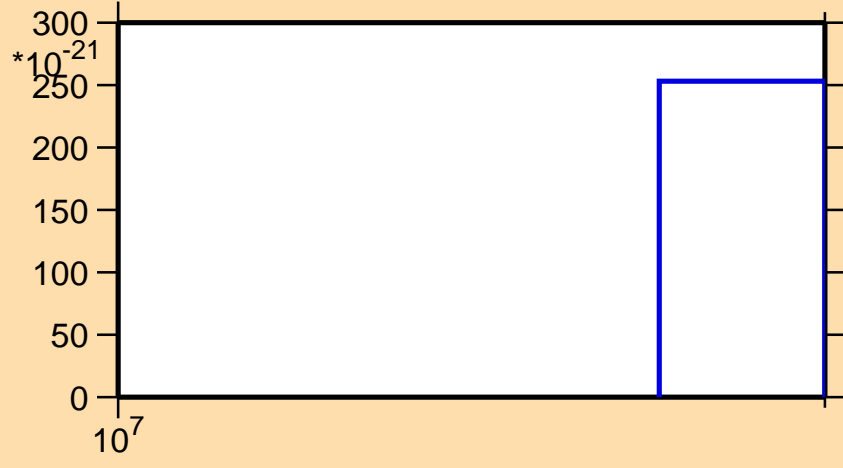
\sigma vs. E for ^{183}\text{Tl} (mt 42)
