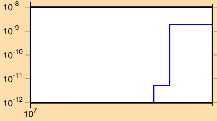
\sigma vs. E for ^{183}\text{Tl}(n,nt)
