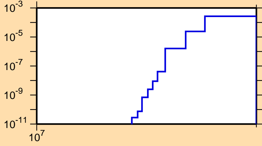
\sigma vs. E for ^{183}\text{Tl}(n,2np)
