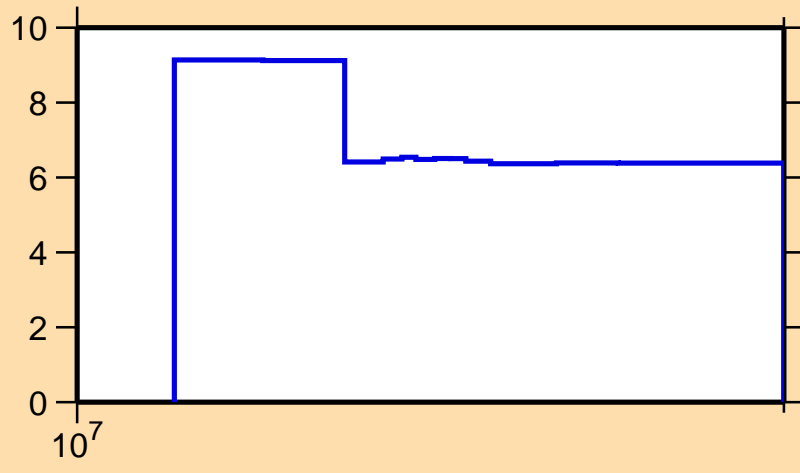
\Delta\sigma/\sigma vs. E for ^{183}\text{Tl}(n,\text{tot.})
