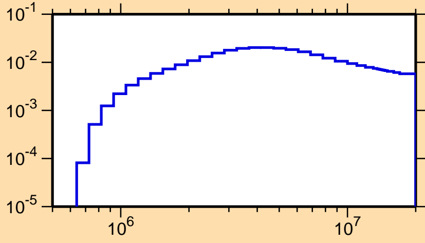
\sigma vs. E for ^{183}\text{Tl}(n,n_2)
