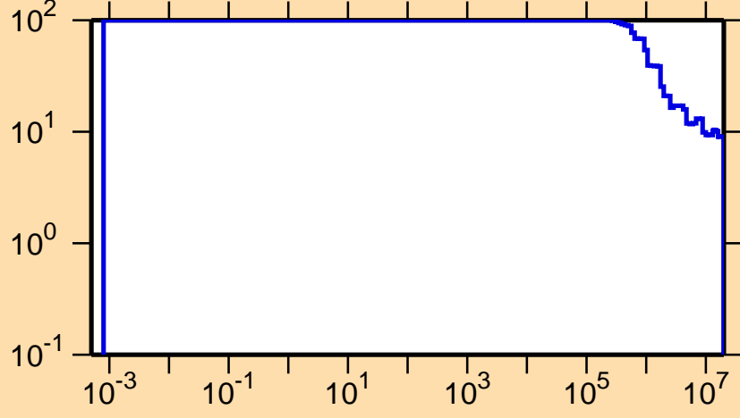
\Delta\sigma/\sigma vs. E for ^{183}\text{Tl}(n,\text{nonel.})
