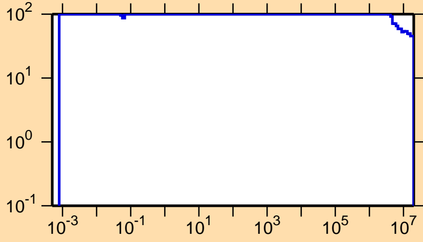
\Delta\sigma/\sigma vs. E for ^{183}\text{Tl}(n,p)
