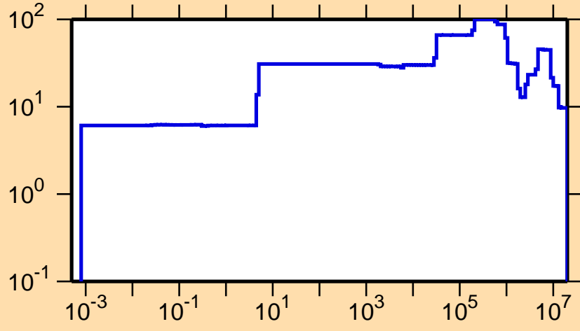
\Delta\sigma/\sigma vs. E for ^{183}\text{Tl}(n,el.)
