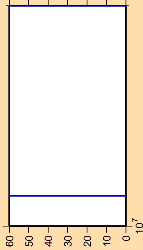
\Delta\sigma/\sigma vs. E for ^{183}\text{Tl}(n,\gamma)
