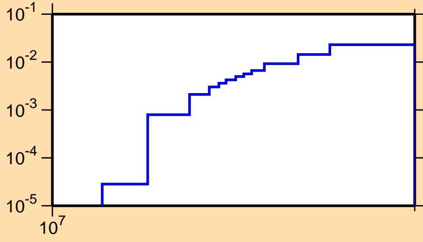
\sigma vs. E for ^{183}\text{Tl}(n,2n)
