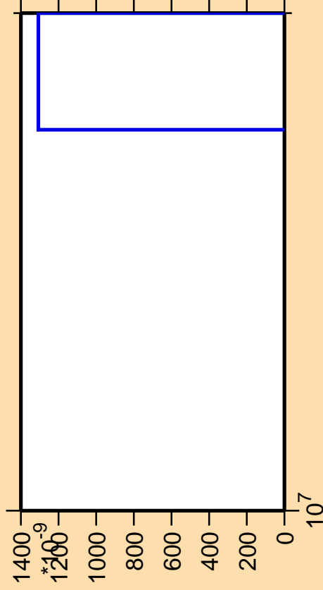
\Delta\sigma/\sigma vs. E for ^{183}\text{Tl} (mt 42)
