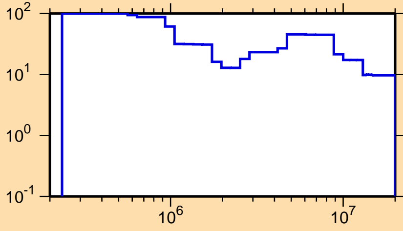
\Delta\sigma/\sigma vs. E for ^{183}\text{Tl}(n,\text{el.})
