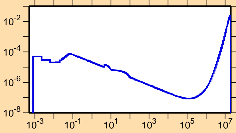
\sigma vs. E for ^{183}\text{Tl}(n,p\alpha)
