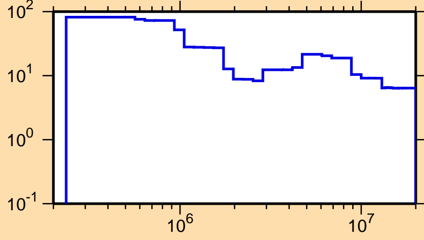
\Delta\sigma/\sigma vs. E for ^{183}\text{Tl}(n,\text{tot.})
