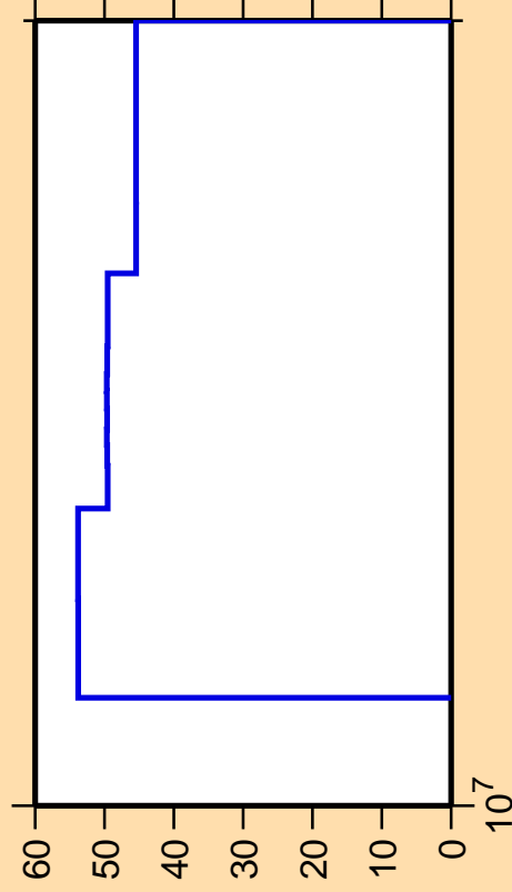
\Delta\sigma/\sigma vs. E for ^{183}\text{Tl}(n,p)
