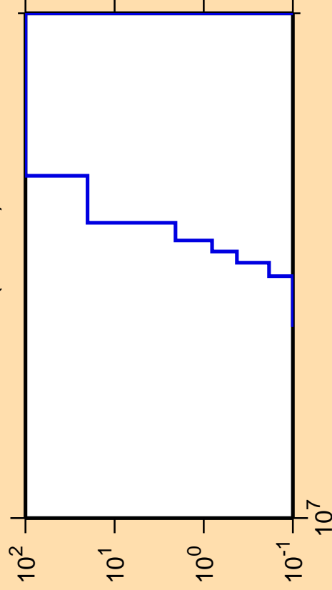
\Delta\sigma/\sigma vs. E for ^{183}\text{Tl} (mt 34)
