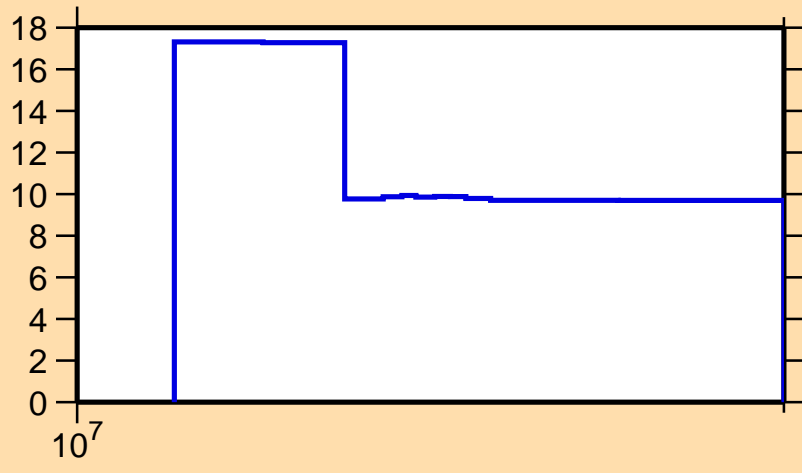
\Delta\sigma/\sigma vs. E for ^{183}\text{Tl}(n,\text{el.})
