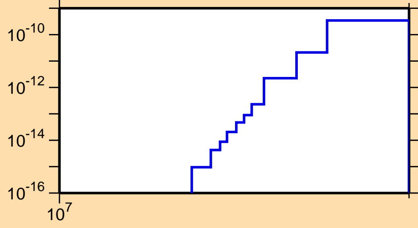
\sigma vs. E for ^{183}\text{Tl} (mt 34)
