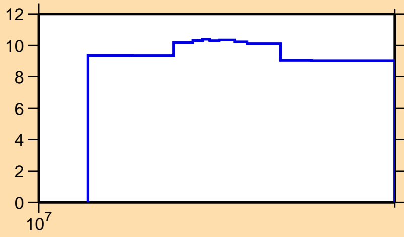
\Delta\sigma/\sigma vs. E for ^{183}\text{Tl}(n,\text{nonel.})
