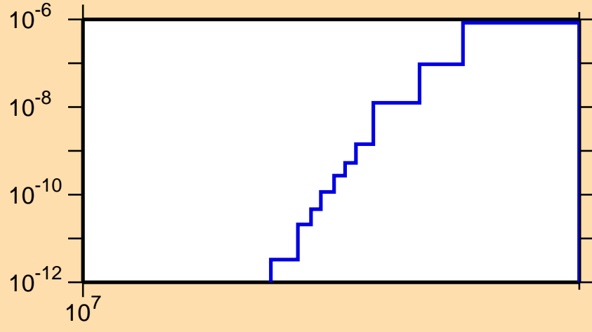
\sigma vs. E for ^{183}\text{Tl}(n,\text{nd})
