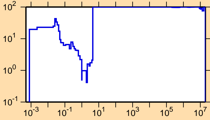
\Delta\sigma/\sigma vs. E for ^{183}\text{Tl}(n,\gamma)
