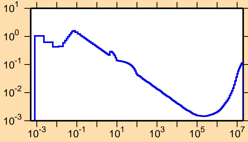
\sigma vs. E for ^{183}\text{Tl}(n,\alpha)
