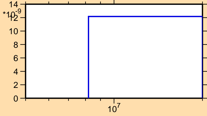
\sigma vs. E for ^{183}\text{Tl}(n,nd)
