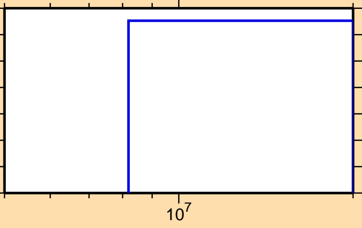
\sigma vs. E for ^{183}\text{Tl}(n,\text{pt})
