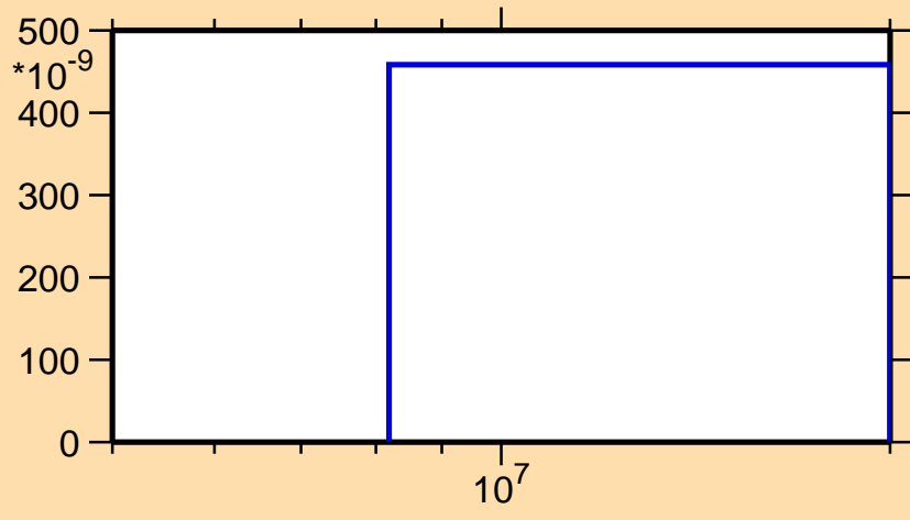
\sigma vs. E for ^{183}\text{Tl}(n,\text{pd})
