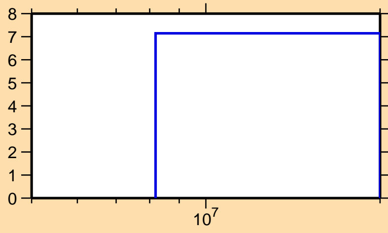
\Delta\sigma/\sigma vs. E for ^{183}\text{Tl}(n,\text{tot.})
