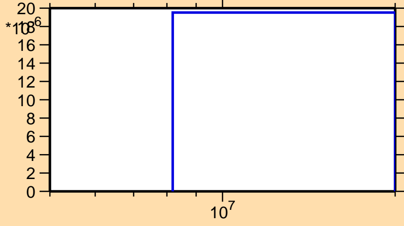
\sigma vs. E for ^{183}\text{Tl}(n,2n\alpha)
