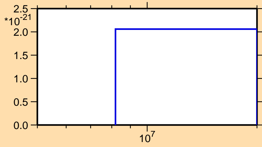
\sigma vs. E for ^{183}\text{Tl} (mt 42)
