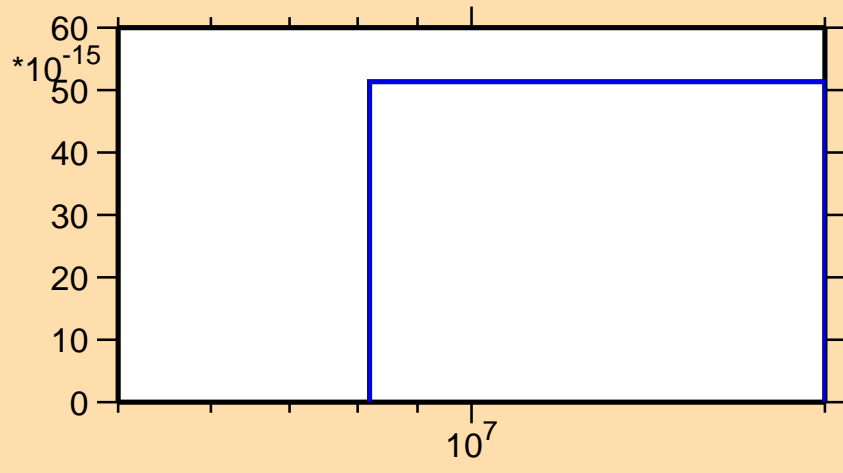
\sigma vs. E for ^{184}\text{Tl}(n,3n)
