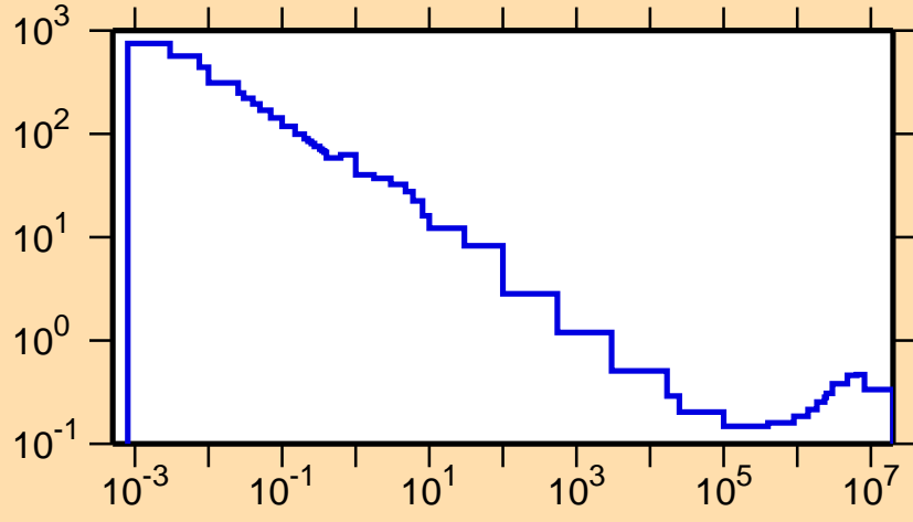
\sigma vs. E for ^{184}\text{Tl}(n,p)
