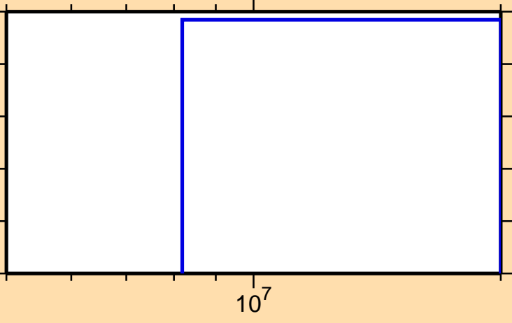
\sigma vs. E for ^{184}\text{Tl}(n,\text{nd})
