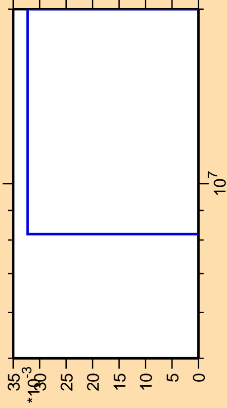
\Delta\sigma/\sigma vs. E for ^{184}\text{Tl}(n,3n)
