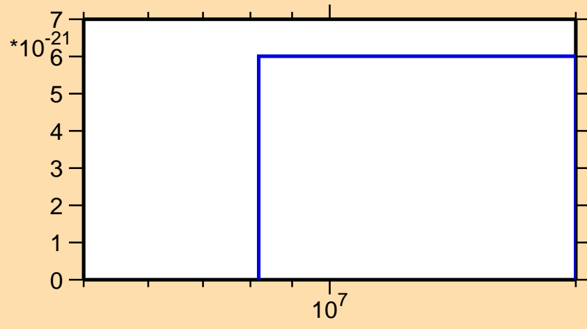
\sigma vs. E for ^{184}\text{Tl} (mt 42)
