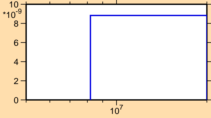
\sigma vs. E for ^{184}\text{Tl}(n,\text{pt})
