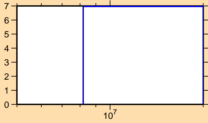
\Delta\sigma/\sigma vs. E for ^{184}\text{Tl}(n,\text{tot.})
