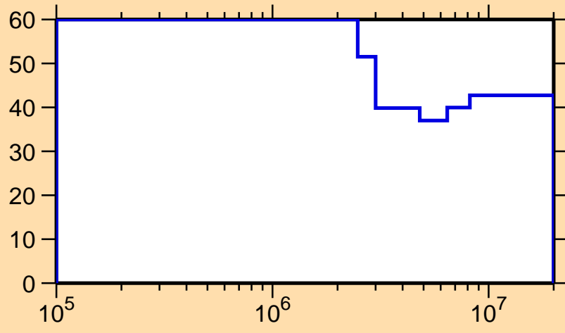
\Delta\sigma/\sigma vs. E for ^{184}\text{Tl}(n,n_1)
