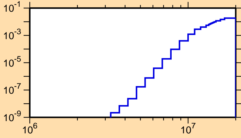
\sigma vs. E for ^{185}\text{Tl}(n,d)
