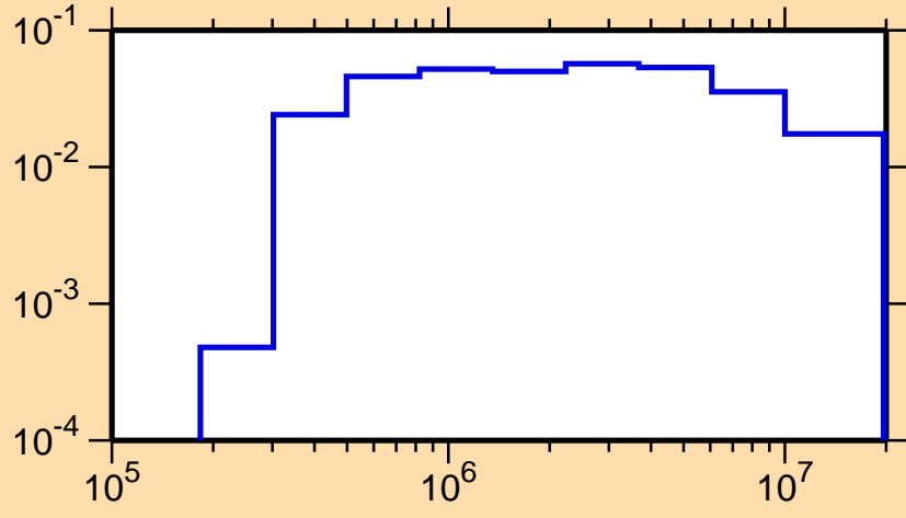
\sigma vs. E for ^{185}\text{Tl}(n,n_2)
