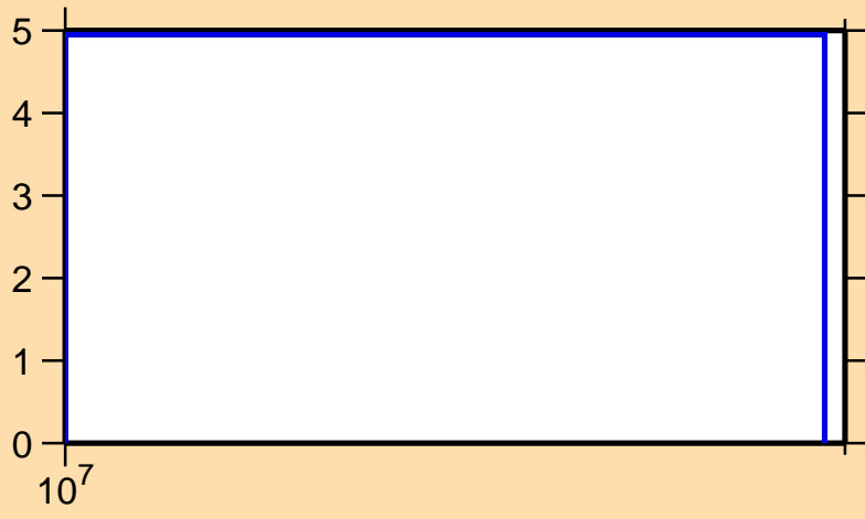
\Delta\sigma/\sigma vs. E for ^{185}\text{Tl}(n,\text{el.})
