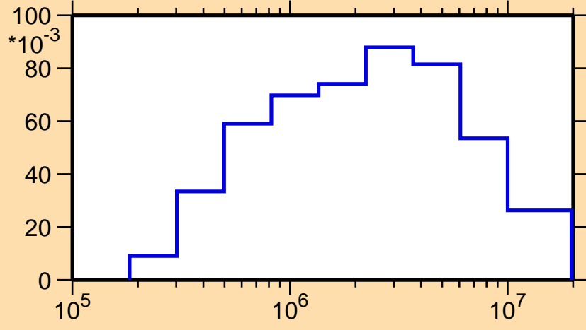
\sigma vs. E for ^{185}\text{Tl}(n,n_1)
