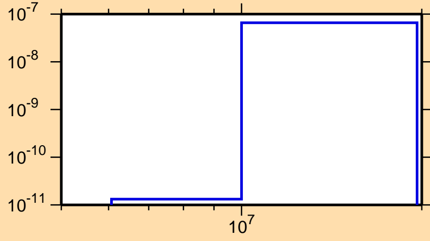
\sigma vs. E for ^{185}\text{Tl}(\text{mt117})
