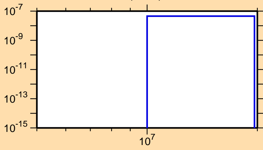
\sigma vs. E for ^{185}\text{Tl}(n,nd)
