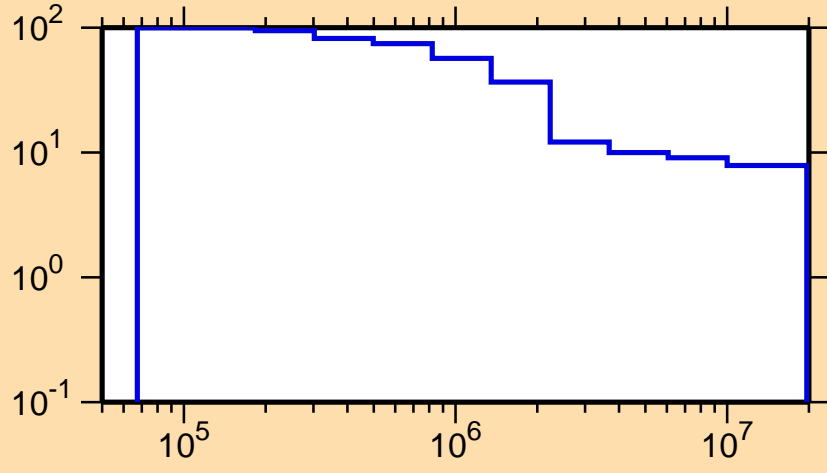
\Delta\sigma/\sigma vs. E for ^{185}\text{Tl}(n,n\text{onel.})
