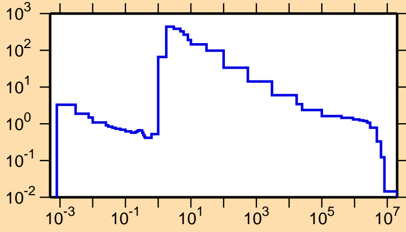
\sigma vs. E for ^{185}\text{Tl}(n,\gamma)
