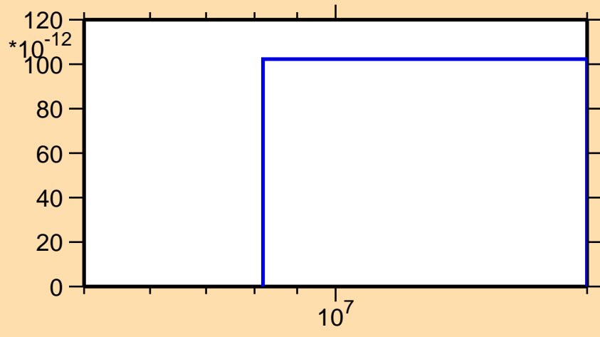
\sigma vs. E for ^{185}\text{Tl}(n,nt)
