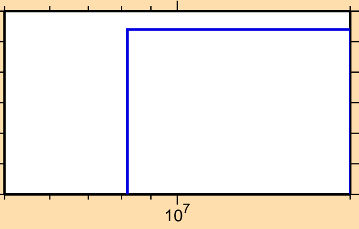
\sigma vs. E for ^{185}\text{Tl}(n,2n)
