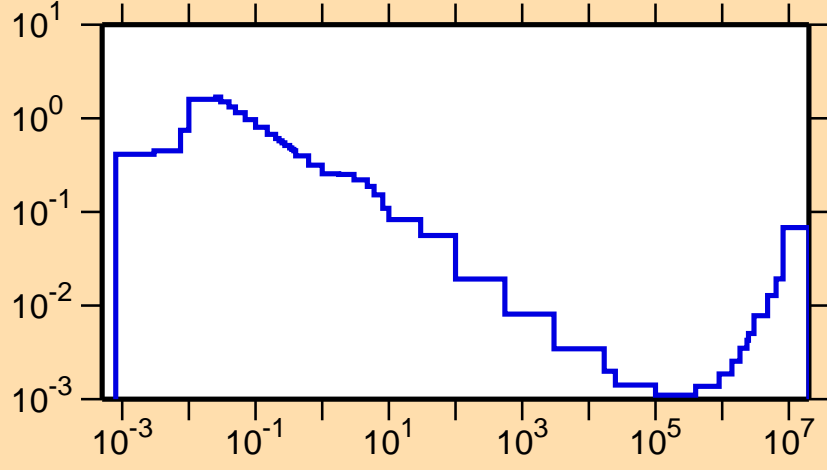
\sigma vs. E for ^{185}\text{Tl}(n,\alpha)
