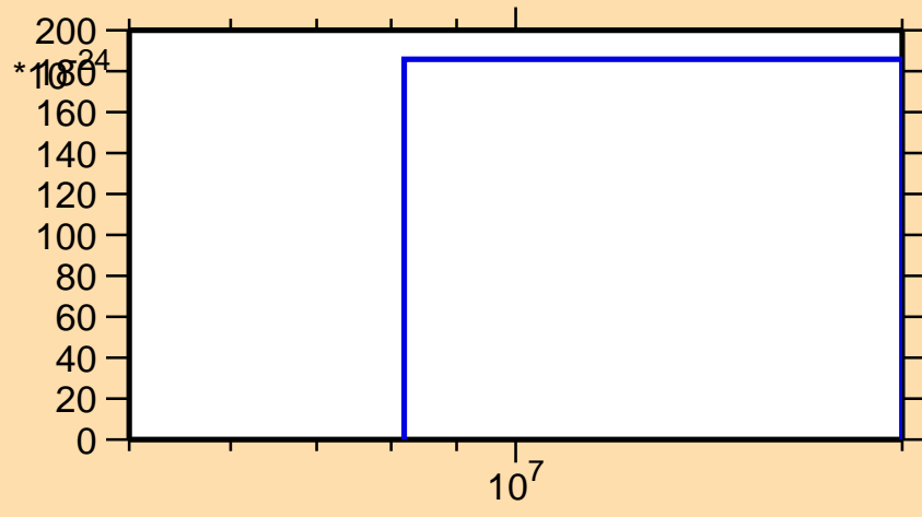
\sigma vs. E for ^{185}\text{Tl} (mt 42)
