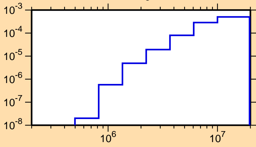
\sigma vs. E for ^{186}\text{Tl}(n,n_3)
