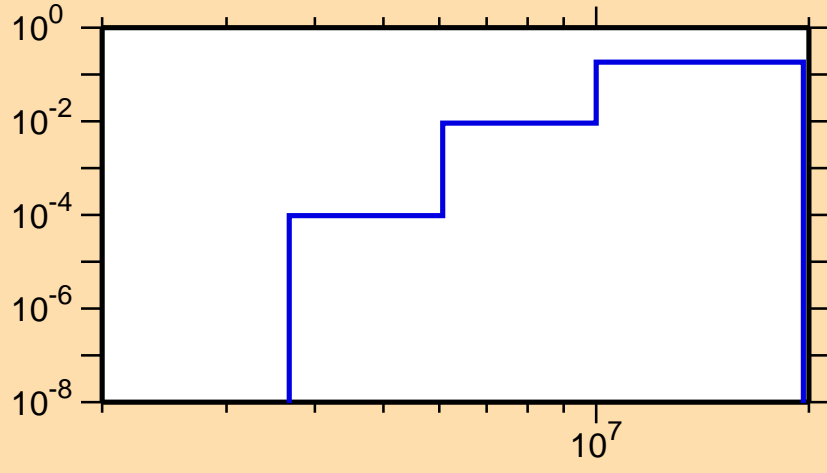
\sigma vs. E for ^{186}\text{Tl}(n,np)
