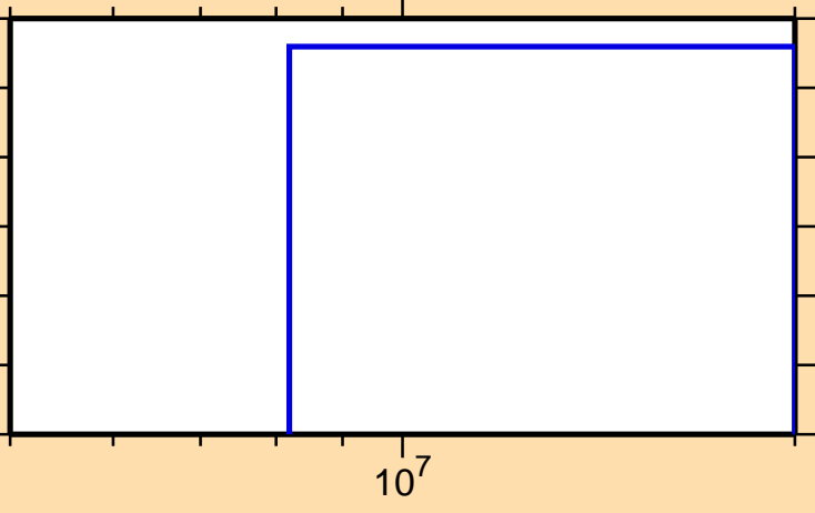
\sigma vs. E for ^{186}\text{Tl}(n,nt)
