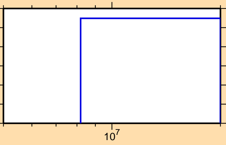
\sigma vs. E for ^{186}\text{Tl}(n,\text{pd})
