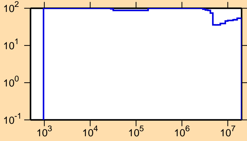
\Delta\sigma/\sigma vs. E for ^{186}\text{Tl}(n,ncont.)
