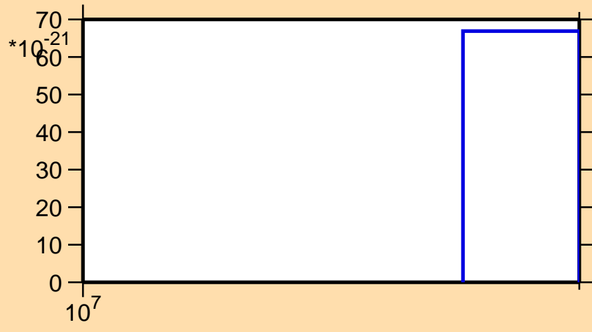
\sigma vs. E for ^{186}\text{Tl} (mt 42)
