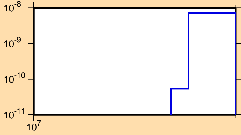
\sigma vs. E for ^{186}\text{Tl}(n,nt)
