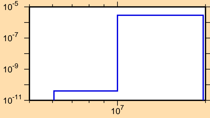
\sigma vs. E for ^{187}\text{Tl} (mt 45)
