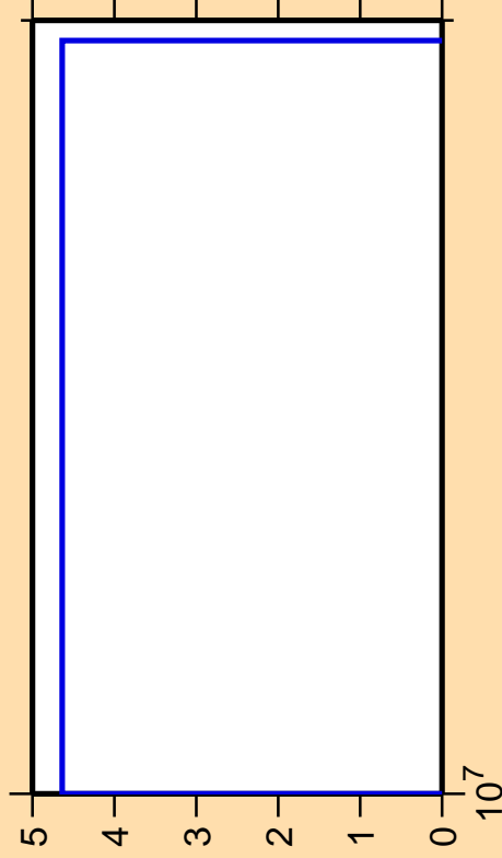
\Delta\sigma/\sigma vs. E for ^{187}\text{Tl} (mt 34)
