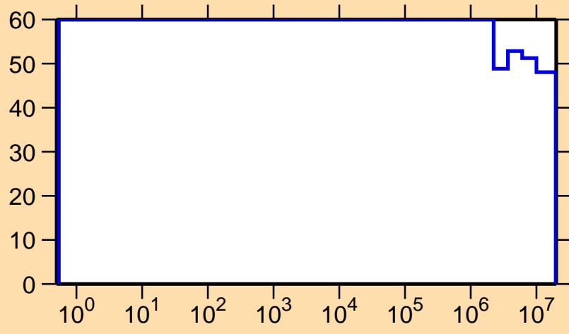
\Delta\sigma/\sigma vs. E for ^{187}\text{Tl}(n,n_1)
