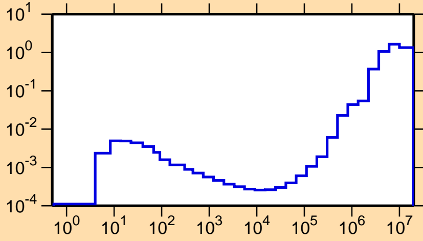
\sigma vs. E for ^{187}\text{Tl}(n,\text{inel.})
