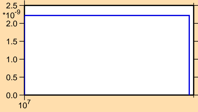
\sigma vs. E for ^{187}\text{Tl}(n,3n\alpha)
