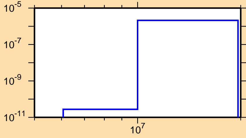
\sigma vs. E for ^{187}\text{Tl}(n,\text{He3})
