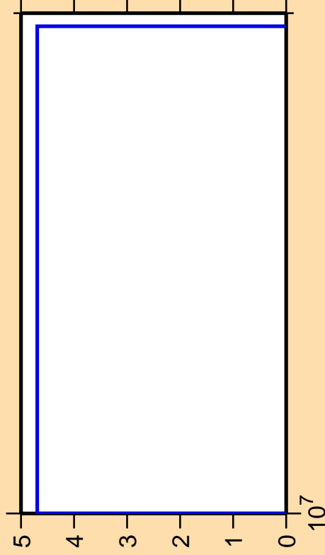
\Delta\sigma/\sigma vs. E for ^{188}\text{Tl}(n,3n\alpha)
