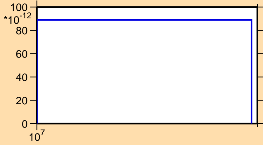
\sigma vs. E for ^{188}\text{Tl}(n,nt)
