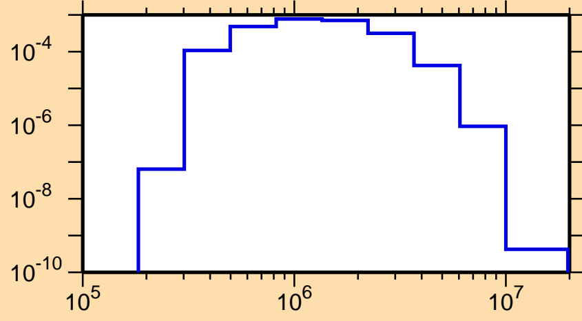
\sigma vs. E for ^{188}\text{Tl}(n,n_4)
