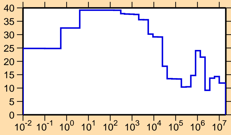
\Delta\sigma/\sigma vs. E for ^{188}\text{Tl}(n,el.)
