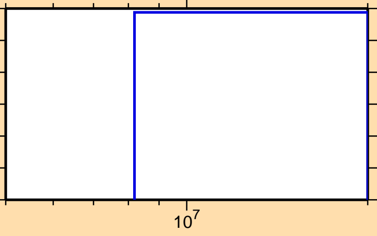
\sigma vs. E for ^{188}\text{Tl}(\text{mt117})
