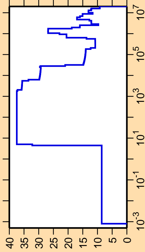
\Delta\sigma/\sigma vs. E for ^{188}\text{Tl}(n,\text{el.})
