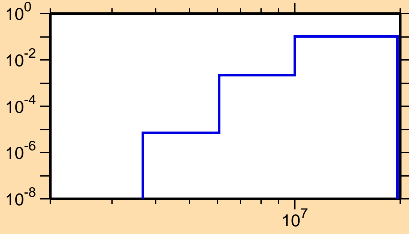
\sigma vs. E for ^{188}\text{Tl}(n,np)
