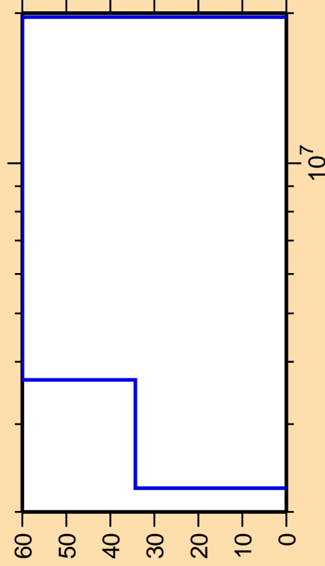
\Delta\sigma/\sigma vs. E for ^{188}\text{Tl}(n,np)
