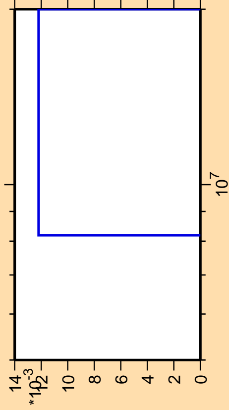
\Delta\sigma/\sigma vs. E for ^{188}\text{Tl}(n,3n\alpha)
