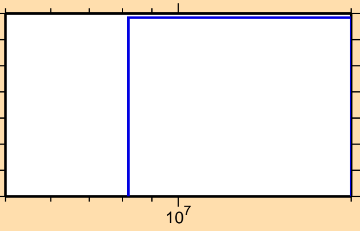
\sigma vs. E for ^{188}\text{Tl}(n,3n)
