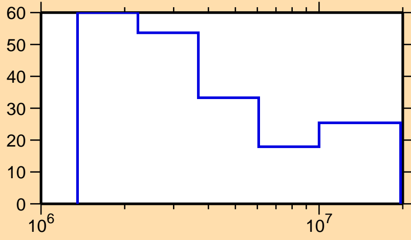
\Delta\sigma/\sigma vs. E for ^{189}\text{Tl}(n,n\text{cont.})
