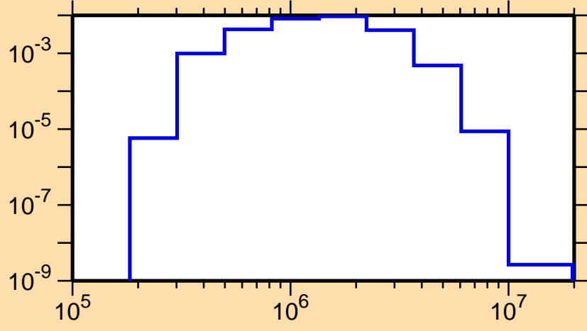
\sigma vs. E for ^{189}\text{Tl}(n,n_1)
