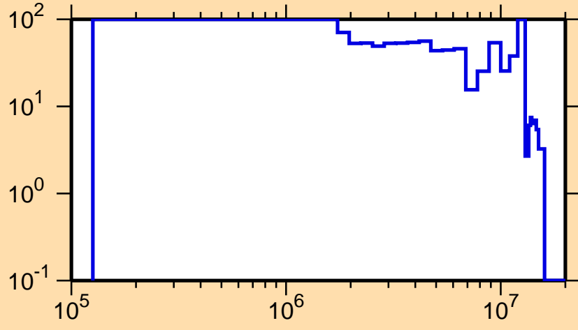
\Delta\sigma/\sigma vs. E for ^{190}\text{Tl}(n,n_1)
