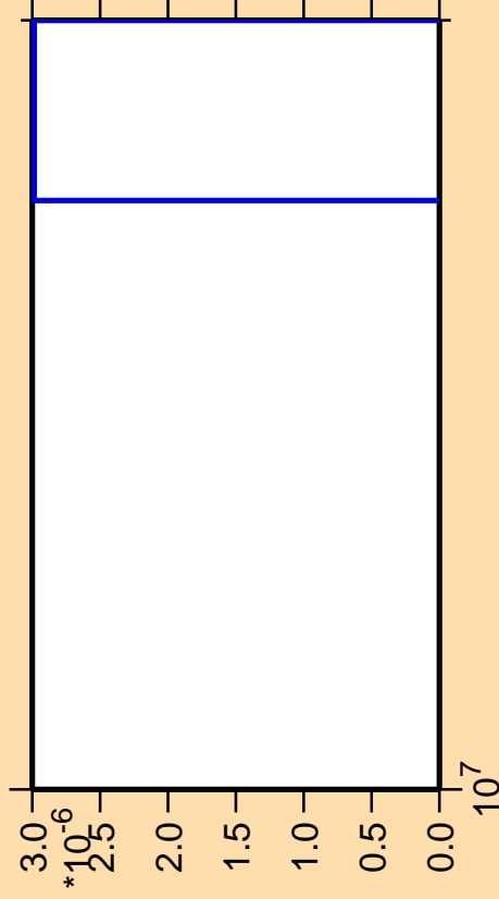
\Delta\sigma/\sigma vs. E for ^{190}\text{Tl} (mt 42)
