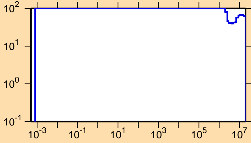
\Delta\sigma/\sigma vs. E for ^{190}\text{Tl}(n,p)
