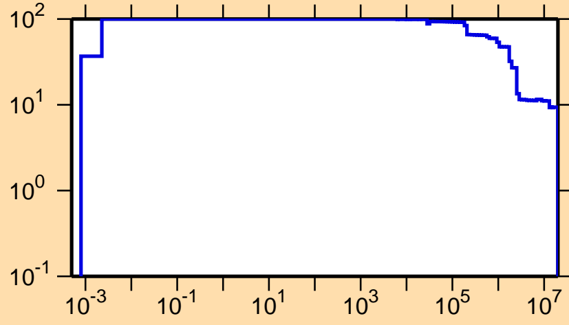
\Delta\sigma/\sigma vs. E for ^{190}\text{Tl}(n,\text{nonel.})
