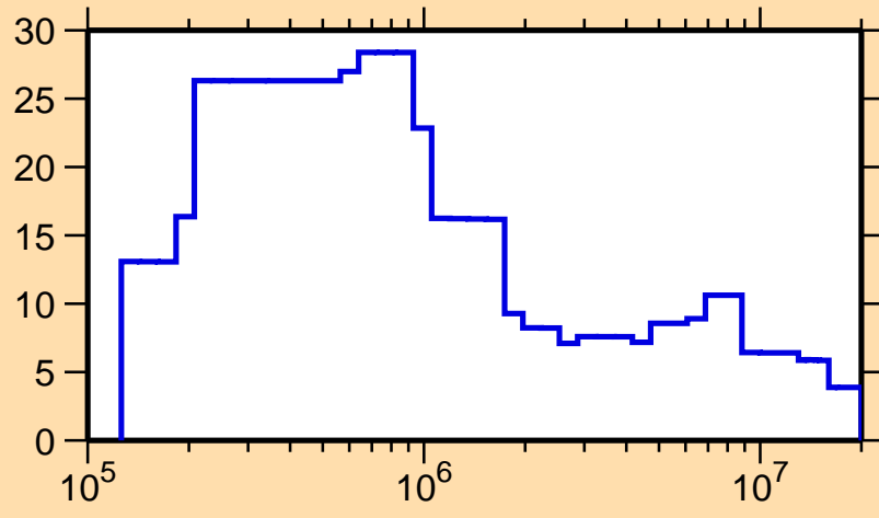
\Delta\sigma/\sigma vs. E for ^{190}\text{Tl}(n,\text{tot.})
