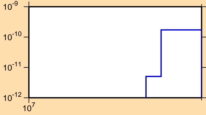
\sigma vs. E for ^{190}\text{Tl}(\text{mt 34})
