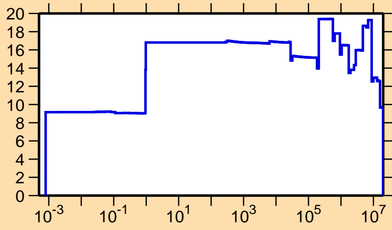
\Delta\sigma/\sigma vs. E for ^{190}\text{Tl}(n,\text{el.})
