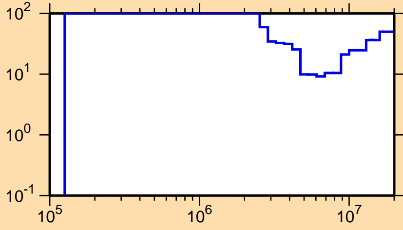
\Delta\sigma/\sigma vs. E for ^{190}\text{Tl}(n,ncont.)
