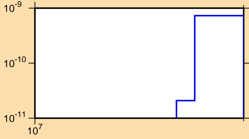
\sigma vs. E for ^{190}\text{Tl}(n,\text{pt})
