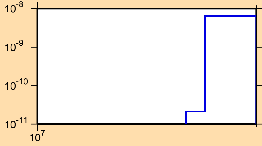
\sigma vs. E for ^{190}\text{Tl}(n,nt)
