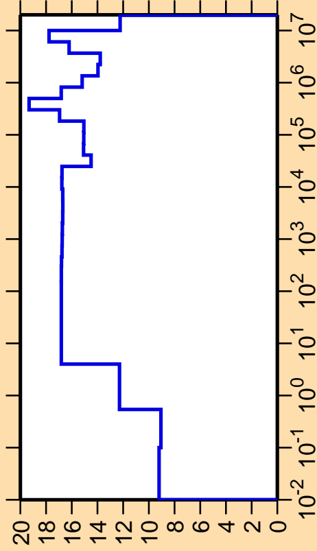
\Delta\sigma/\sigma vs. E for ^{190}\text{Tl}(n,\text{el.})
