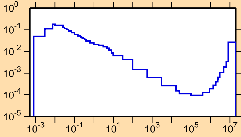
\sigma vs. E for ^{190}\text{Tl}(n,\alpha)
