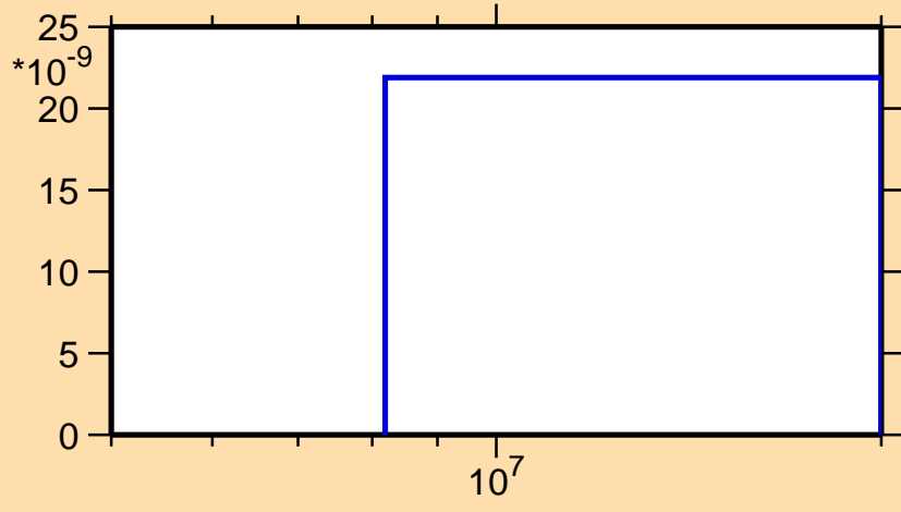
\sigma vs. E for ^{190}\text{Tl} (mt 45)
