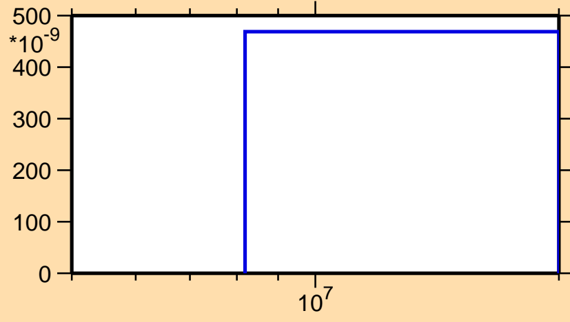
\sigma vs. E for ^{190}\text{Tl}(n,\text{He3})
