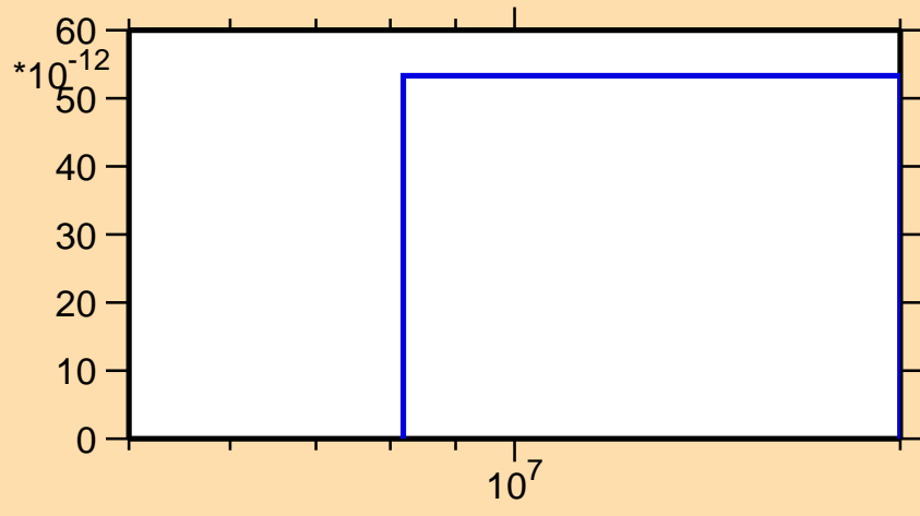
\sigma vs. E for ^{190}\text{Tl}(n,nt)
