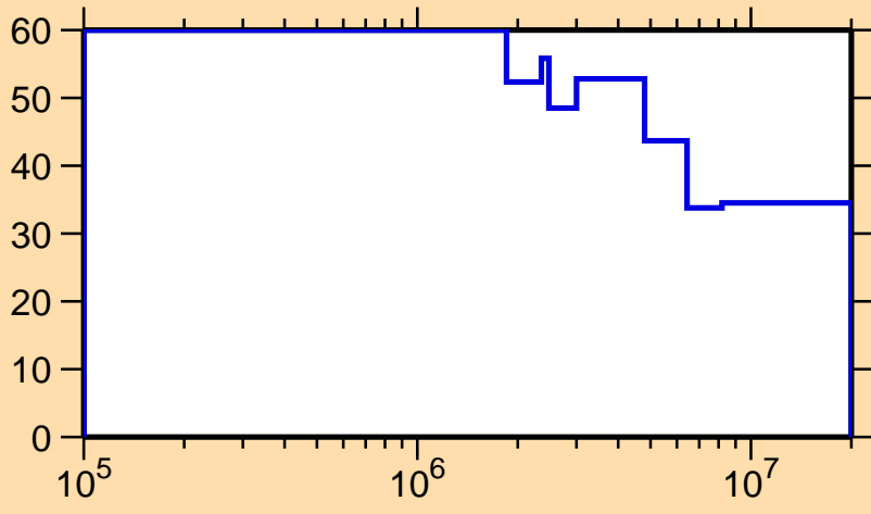
\Delta\sigma/\sigma vs. E for ^{190}\text{Tl}(n,n_1)
