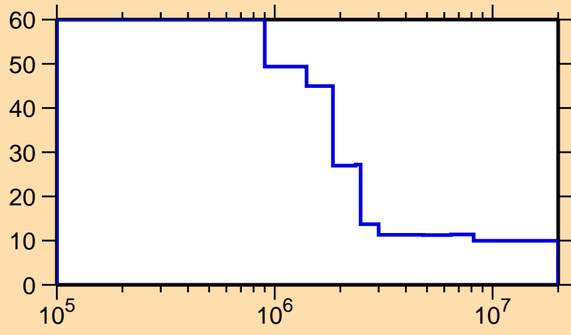
\Delta\sigma/\sigma vs. E for ^{190}\text{Tl}(n,\text{nonel.})
