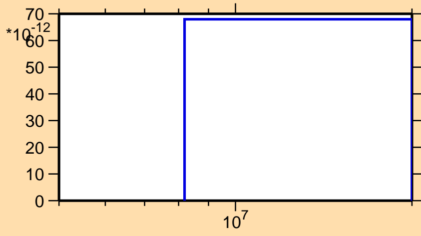
\sigma vs. E for ^{190}\text{Tl}(n,\text{pd})
