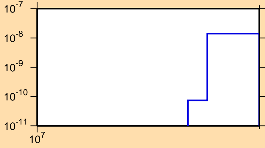
\sigma vs. E for ^{191}\text{Tl}(n,nt)
