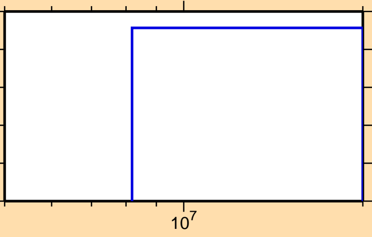
\sigma vs. E for ^{191}\text{Tl}(n,\text{He3})
