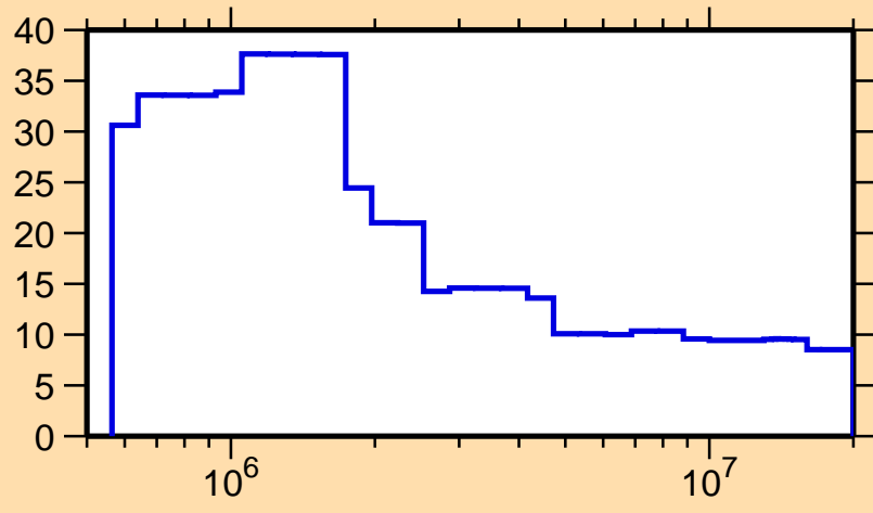
\Delta\sigma/\sigma vs. E for ^{191}\text{Tl}(n,\text{nonel.})
