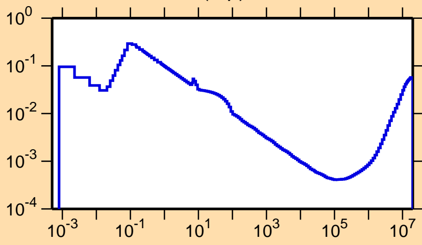
\sigma vs. E for ^{191}\text{Tl}(n,p)
