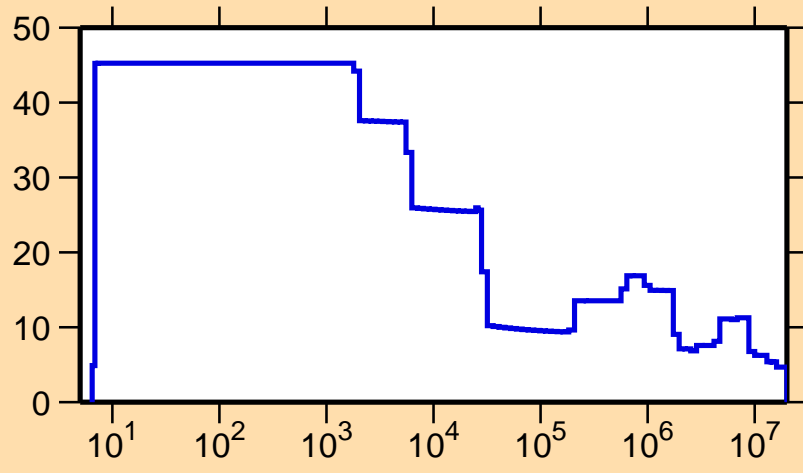
\Delta\sigma/\sigma vs. E for ^{191}\text{Tl}(n,\text{tot.})
