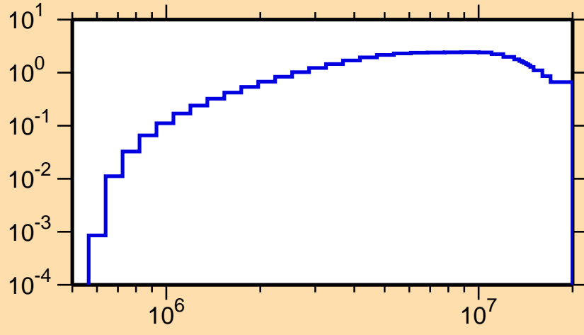
\sigma vs. E for ^{191}\text{Tl}(n,n\text{cont.})
