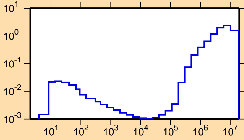
\sigma vs. E for ^{191}\text{Tl}(n,\text{inel.})
