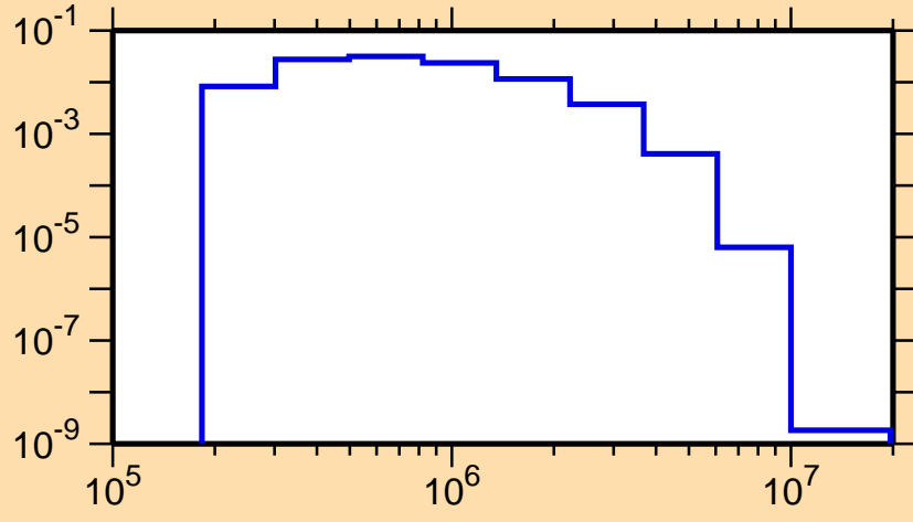
\sigma vs. E for ^{191}\text{Tl}(n,n_4)
