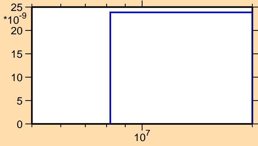
\sigma vs. E for ^{191}\text{Tl}(n,2n\alpha)
