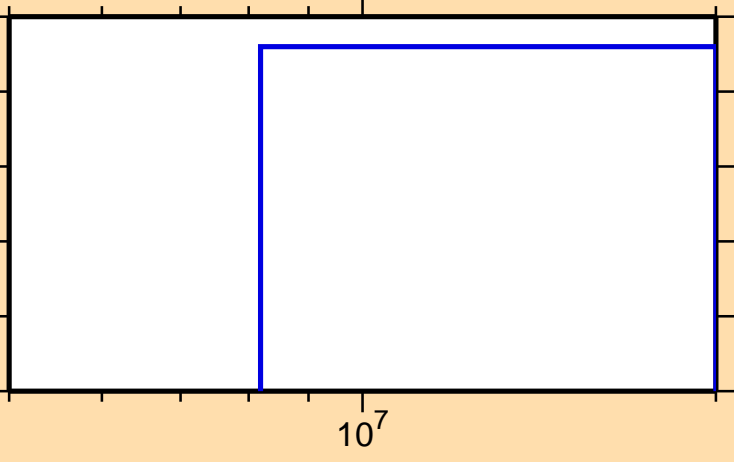
\sigma vs. E for ^{191}\text{Tl}(n,\text{He}3)
