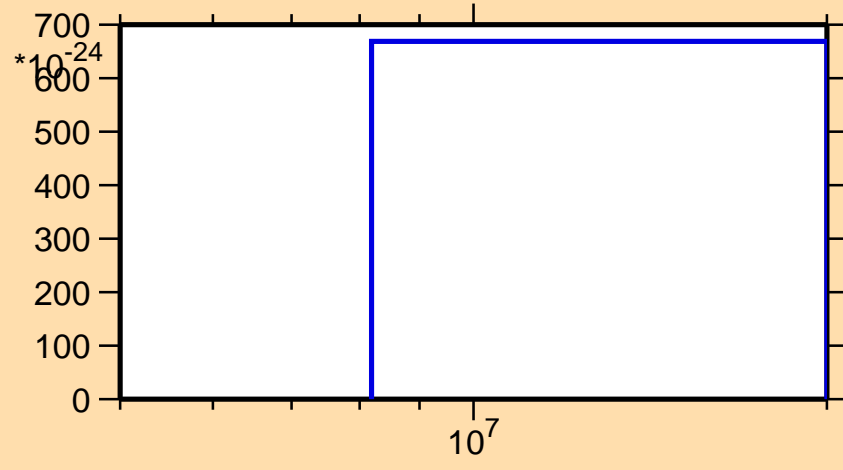
\sigma vs. E for ^{191}\text{Tl} (mt 42)
