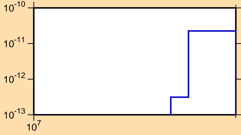
\sigma vs. E for ^{192}\text{Tl} (mt 34)
