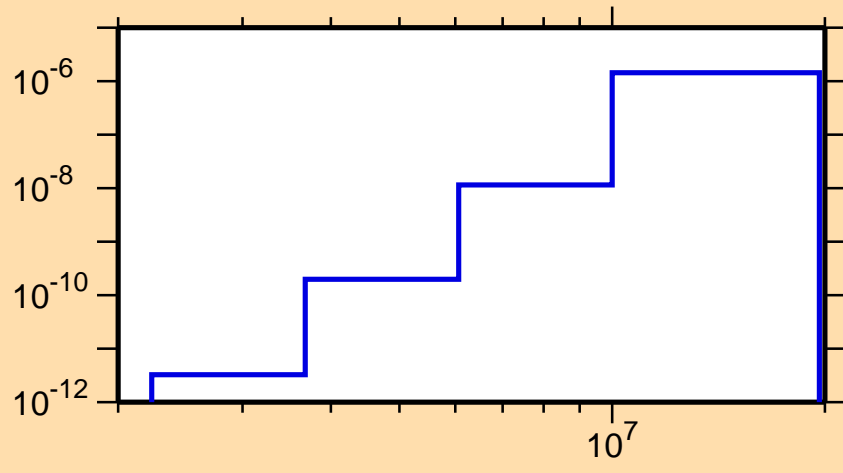
\sigma vs. E for ^{192}\text{Tl}(n,p\alpha)
