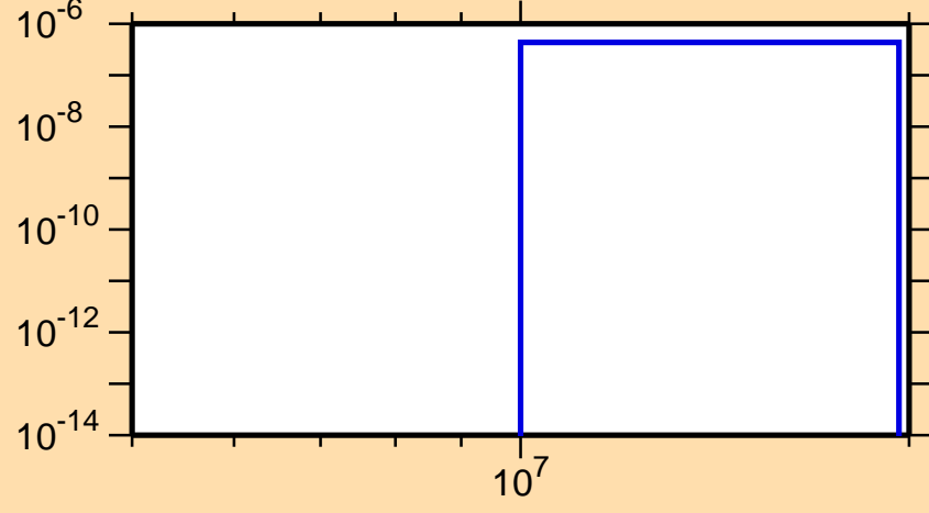
\sigma vs. E for ^{192}\text{Tl}(n,nd)
