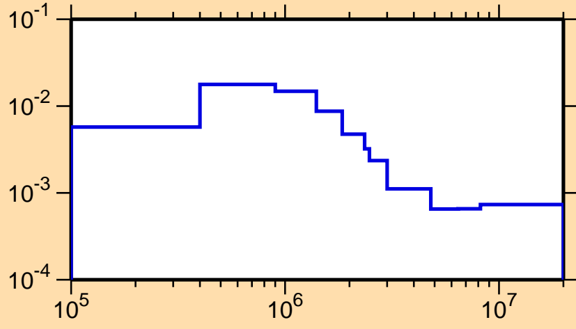
\sigma vs. E for ^{192}\text{Tl}(n,n_2)
