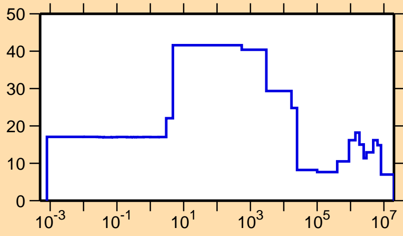
\Delta\sigma/\sigma vs. E for ^{192}\text{Tl}(n,el.)
