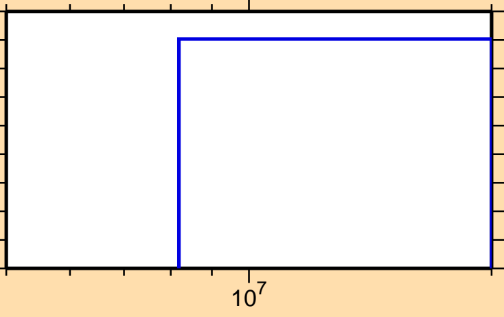
\sigma vs. E for ^{192}\text{Tl}(n,2np)
