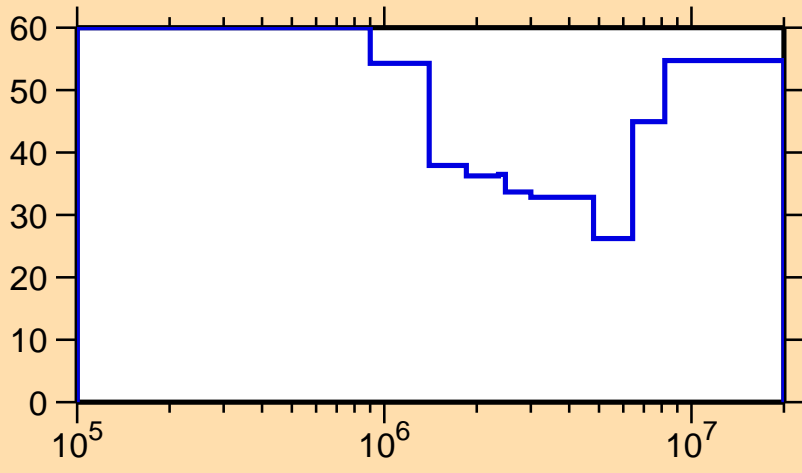
\Delta\sigma/\sigma vs. E for ^{192}\text{Tl}(n,n_1)
