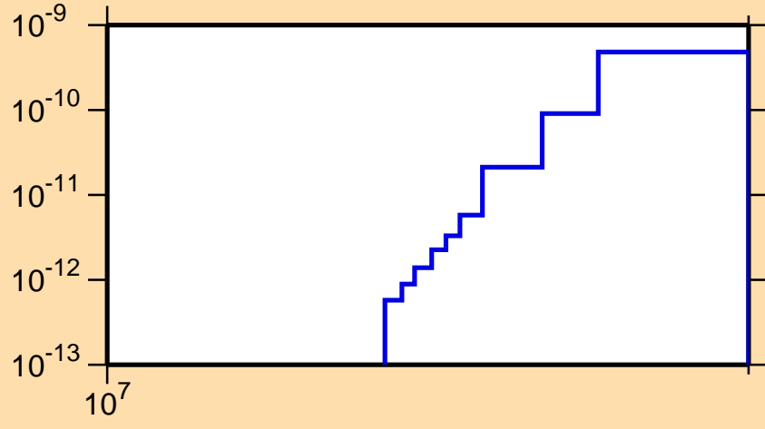
\sigma vs. E for ^{192}\text{Tl}(\text{mt117})
