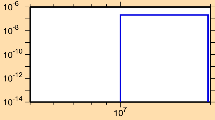
\sigma vs. E for ^{192}\text{Tl}(n,nd)
