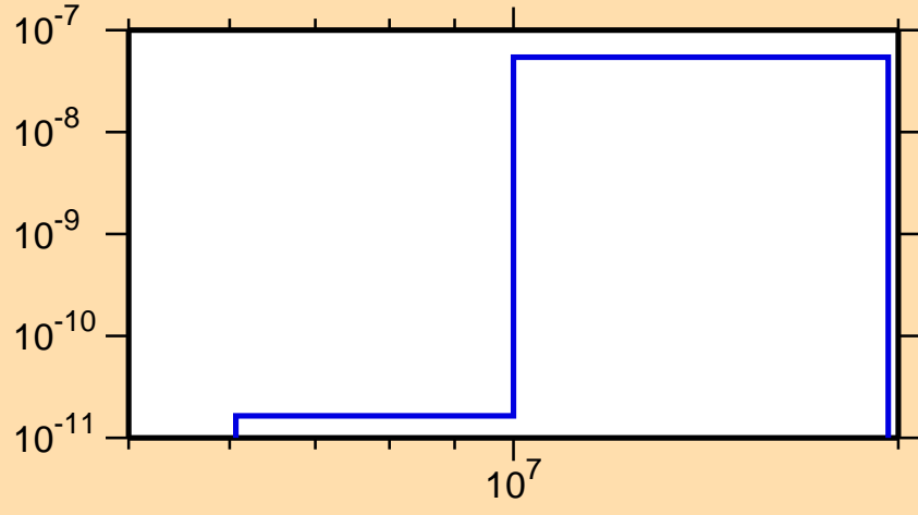
\sigma vs. E for ^{193}\text{Tl}(n,p\alpha)
