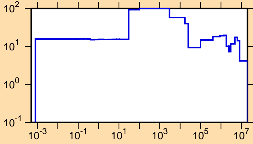
\Delta\sigma/\sigma vs. E for ^{193}\text{Tl}(n,el.)
