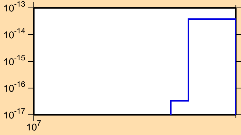
\sigma vs. E for ^{193}\text{Tl}(n,\text{pt})
