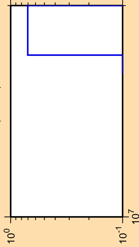
\Delta\sigma/\sigma vs. E for ^{193}\text{Tl} (mt 34)
