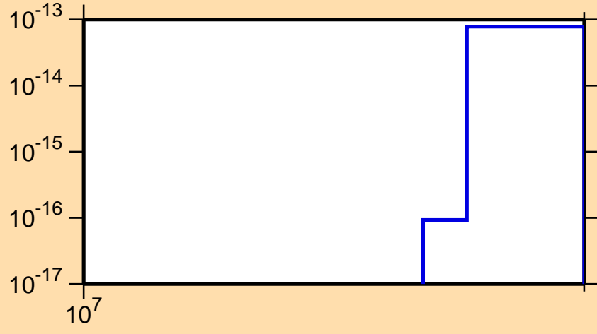
\sigma vs. E for ^{193}\text{Tl} (mt 34)
