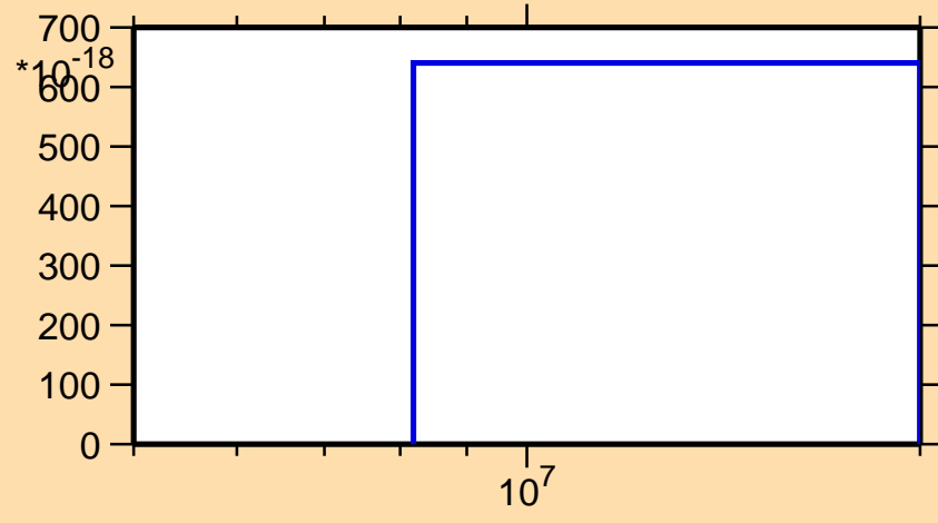
\sigma vs. E for ^{193}\text{Tl} (mt 34)
