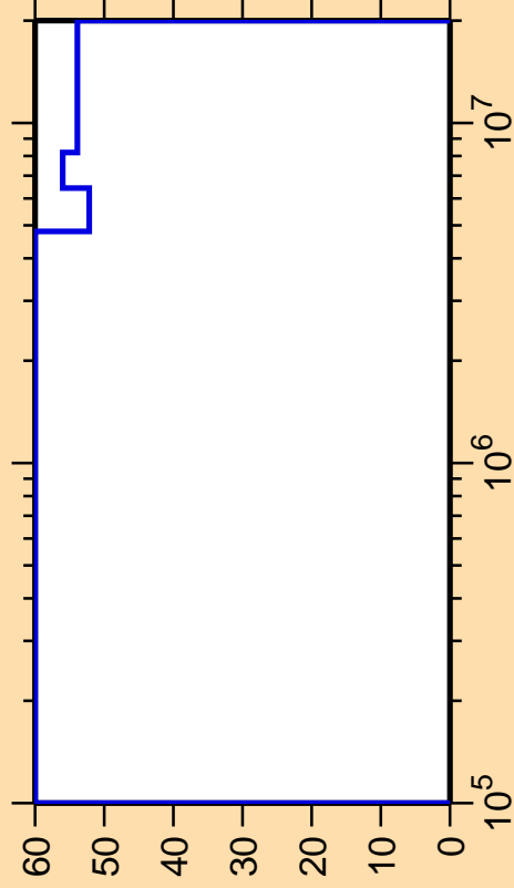
\Delta\sigma/\sigma vs. E for ^{193}\text{Tl}(n,n_4)
