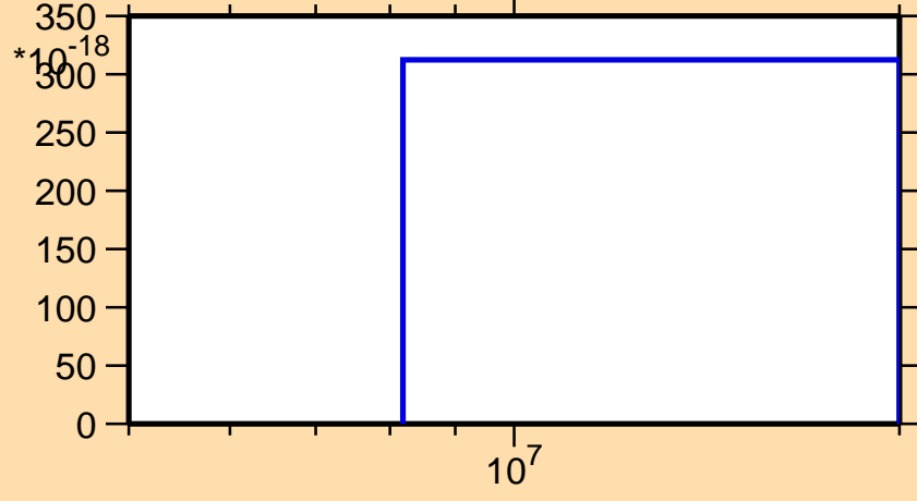
\sigma vs. E for ^{193}\text{Tl}(n,\text{pt})
