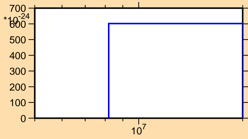
\sigma vs. E for ^{193}\text{Tl} (mt 42)
