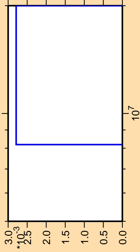
\Delta\sigma/\sigma vs. E for ^{193}\text{Tl}(n,\text{pt})
