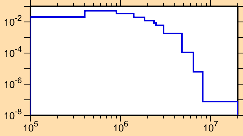
\sigma vs. E for ^{193}\text{Tl}(n,n_4)
