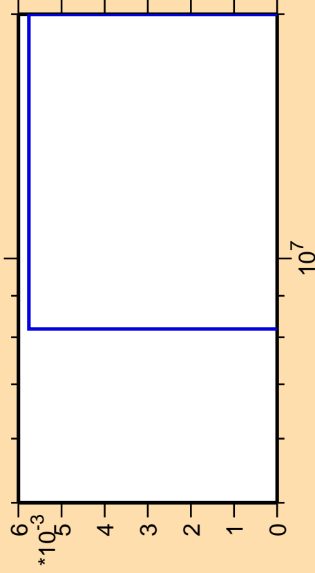
\Delta\sigma/\sigma vs. E for ^{193}\text{Tl} (mt 34)
