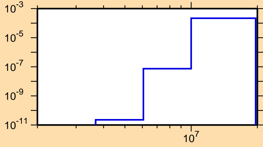
\sigma vs. E for ^{194}\text{Tl}(n,n\alpha)
