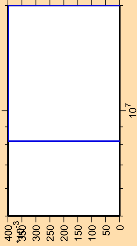
\Delta\sigma/\sigma vs. E for ^{194}\text{Tl}(n,\text{pd})
