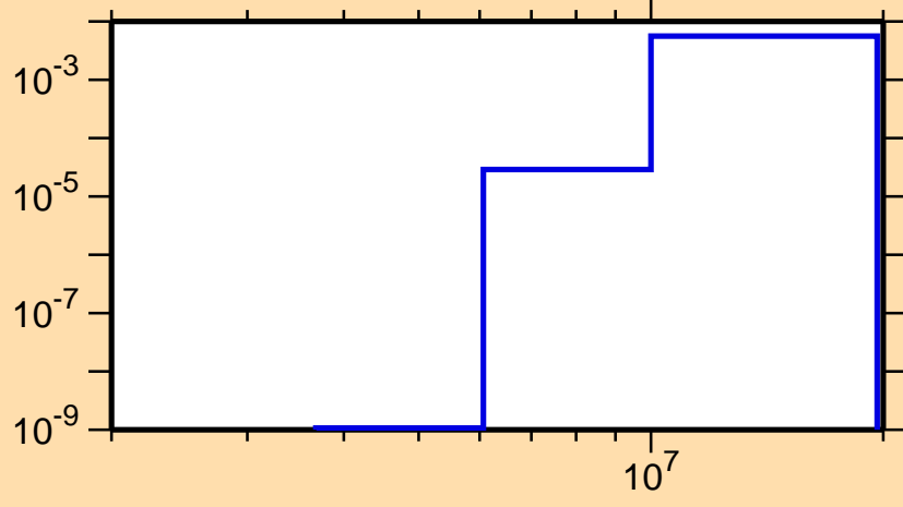
\sigma vs. E for ^{194}\text{Tl}(n,np)
